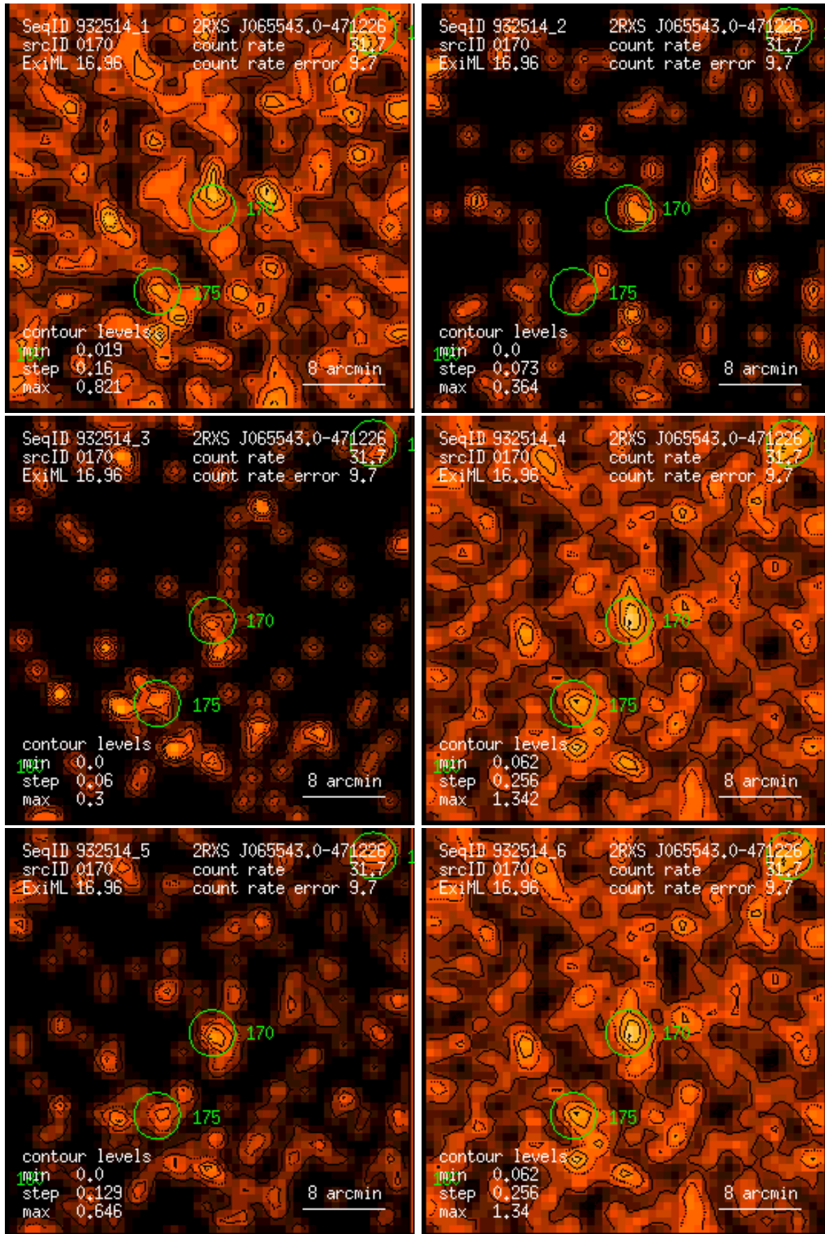
Figure 170: RASS 932514: detection 0170: band rate images, Gaussian filter: (1) PSPC channels 11 – 41, (2) 52 – 90, (3) 91 – 201, (4) 11 – 235, (5) 52 – 201, (6) 11 – 201. Broad band rates in counts/ks. Band rate contour levels in counts/ks/arcmin 2 .
