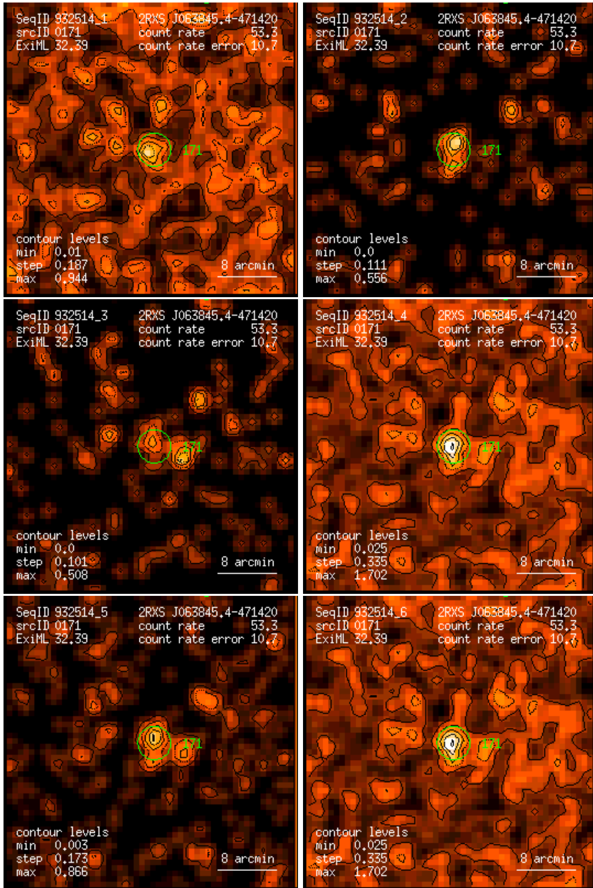
Figure 171: RASS 932514: detection 0171: band rate images, Gaussian filter: (1) PSPC channels 11 – 41, (2) 52 – 90, (3) 91 – 201, (4) 11 – 235, (5) 52 – 201, (6) 11 – 201. Broad band rates in counts/ks. Band rate contour levels in counts/ks/arcmin 2 .
