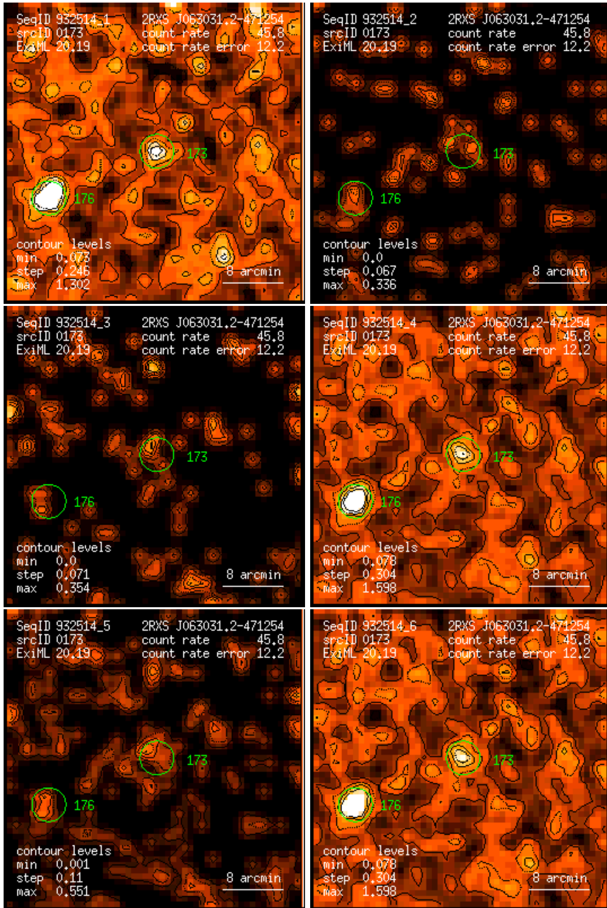
Figure 173: RASS 932514: detection 0173: band rate images, Gaussian filter: (1) PSPC channels 11 – 41, (2) 52 – 90, (3) 91 – 201, (4) 11 – 235, (5) 52 – 201, (6) 11 – 201. Broad band rates in counts/ks. Band rate contour levels in counts/ks/arcmin 2 .
