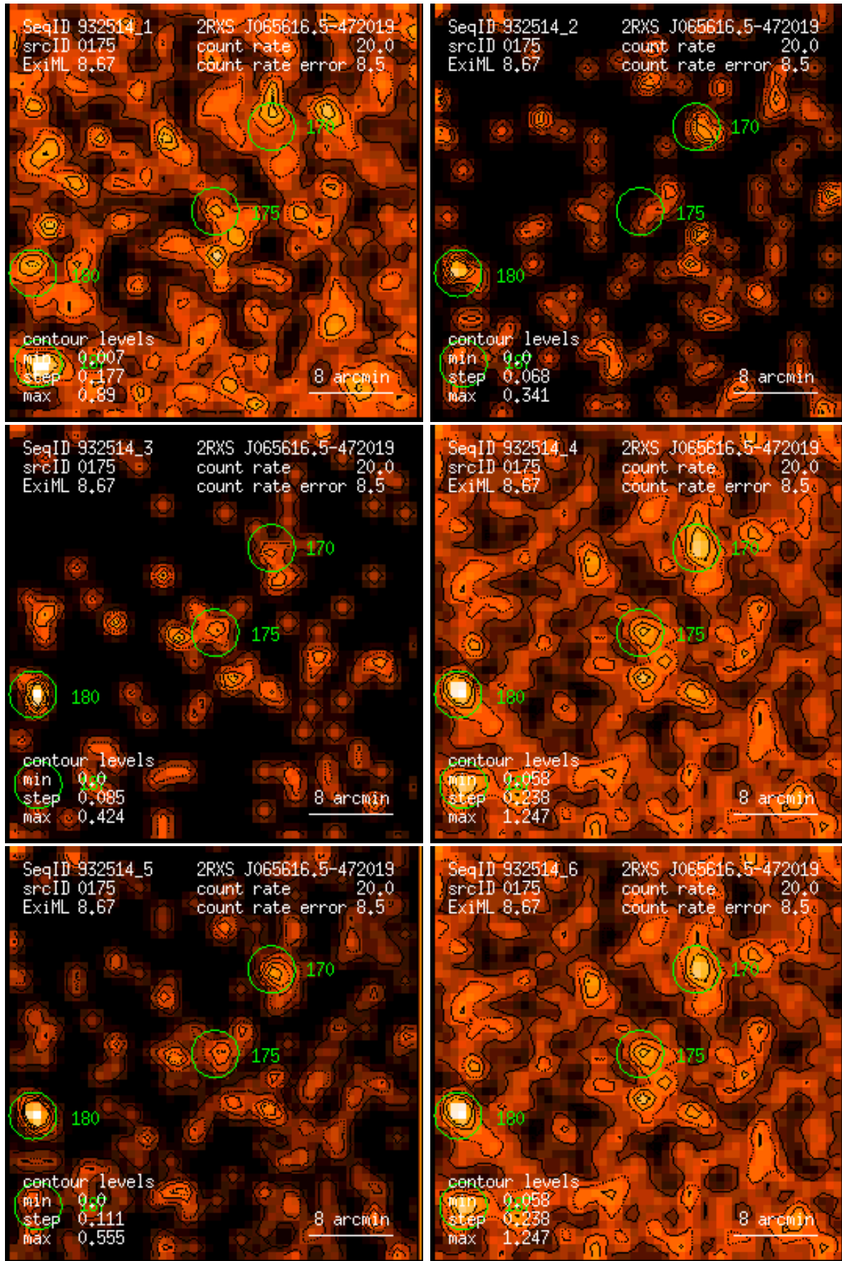
Figure 175: RASS 932514: detection 0175: band rate images, Gaussian filter: (1) PSPC channels 11 – 41, (2) 52 – 90, (3) 91 – 201, (4) 11 – 235, (5) 52 – 201, (6) 11 – 201. Broad band rates in counts/ks. Band rate contour levels in counts/ks/arcmin 2 .
