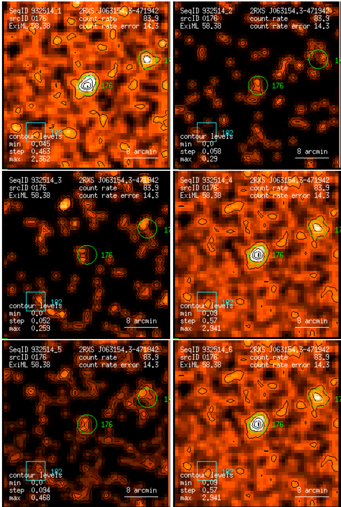
Figure 176: RASS 932514: detection 0176: band rate images, Gaussian filter: (1) PSPC channels 11 – 41, (2) 52 – 90, (3) 91 – 201, (4) 11 – 235, (5) 52 – 201, (6) 11 – 201. Broad band rates in counts/ks. Band rate contour levels in counts/ks/arcmin 2 .
