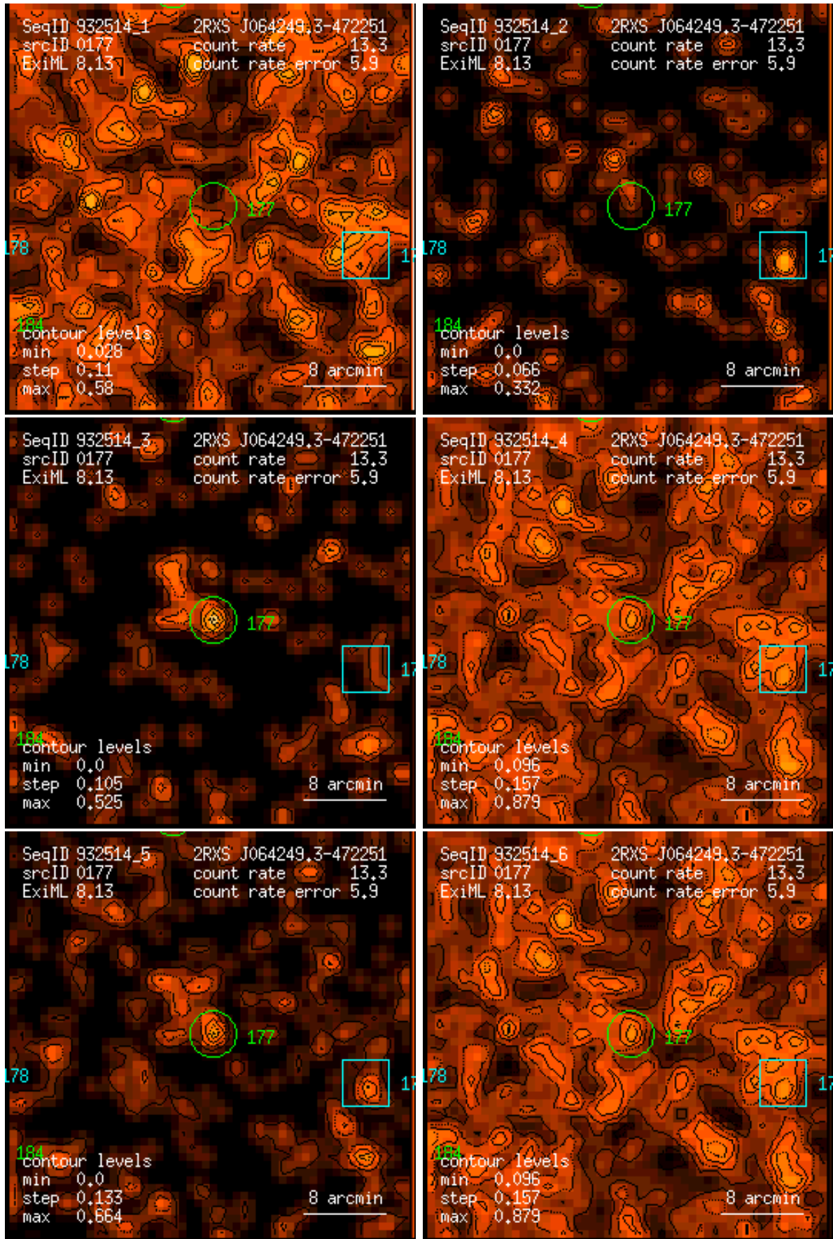
Figure 177: RASS 932514: detection 0177: band rate images, Gaussian filter: (1) PSPC channels 11 – 41, (2) 52 – 90, (3) 91 – 201, (4) 11 – 235, (5) 52 – 201, (6) 11 – 201. Broad band rates in counts/ks. Band rate contour levels in counts/ks/arcmin 2 .
