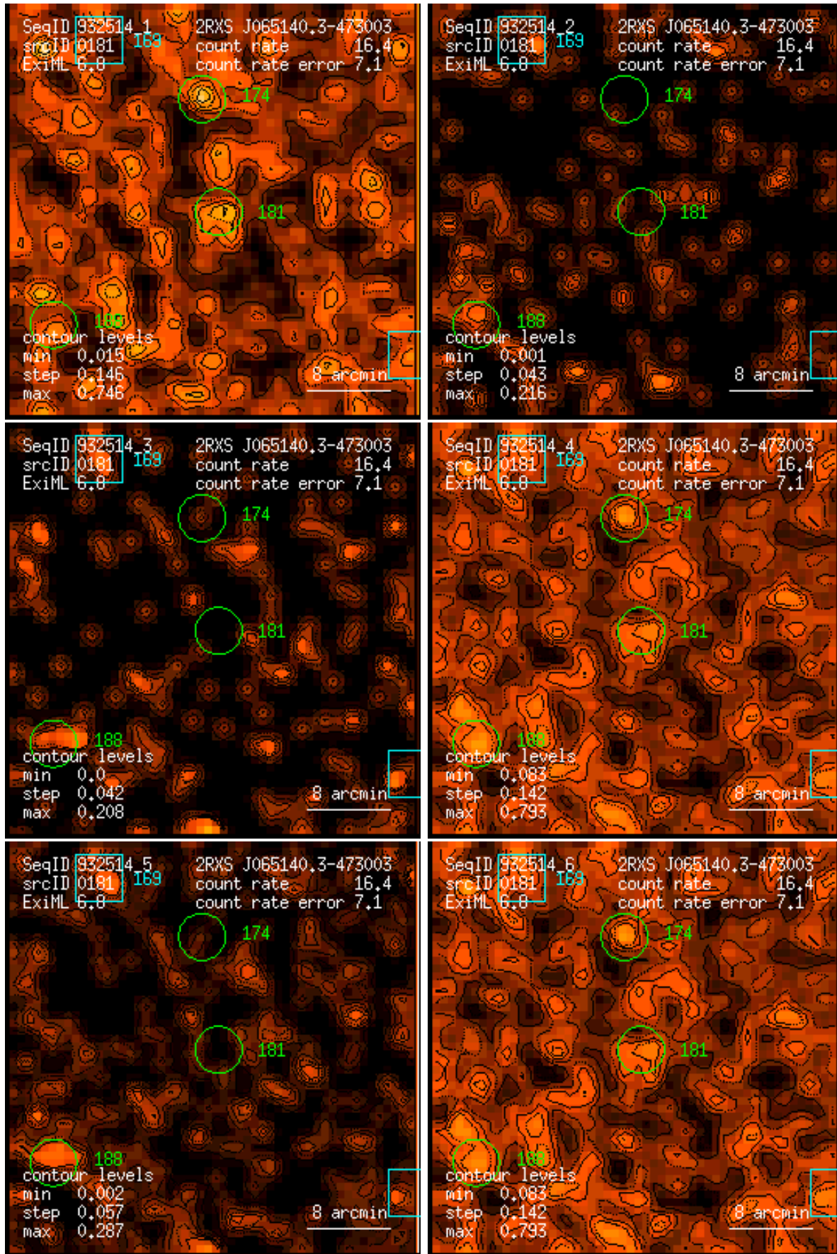
Figure 181: RASS 932514: detection 0181: band rate images, Gaussian filter: (1) PSPC channels 11 – 41, (2) 52 – 90, (3) 91 – 201, (4) 11 – 235, (5) 52 – 201, (6) 11 – 201. Broad band rates in counts/ks. Band rate contour levels in counts/ks/arcmin 2 .
