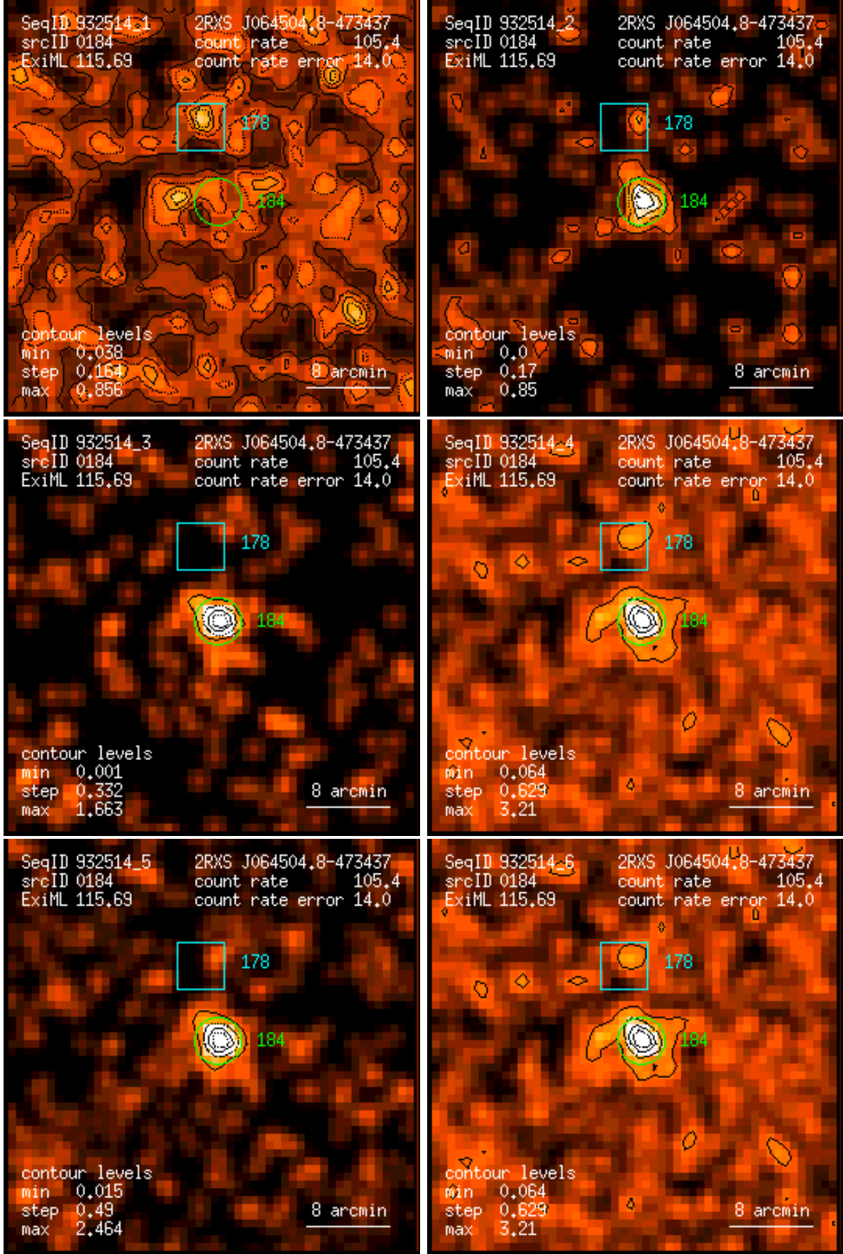
Figure 184: RASS 932514: detection 0184: band rate images, Gaussian filter: (1) PSPC channels 11 – 41, (2) 52 – 90, (3) 91 – 201, (4) 11 – 235, (5) 52 – 201, (6) 11 – 201. Broad band rates in counts/ks. Band rate contour levels in counts/ks/arcmin 2 .
