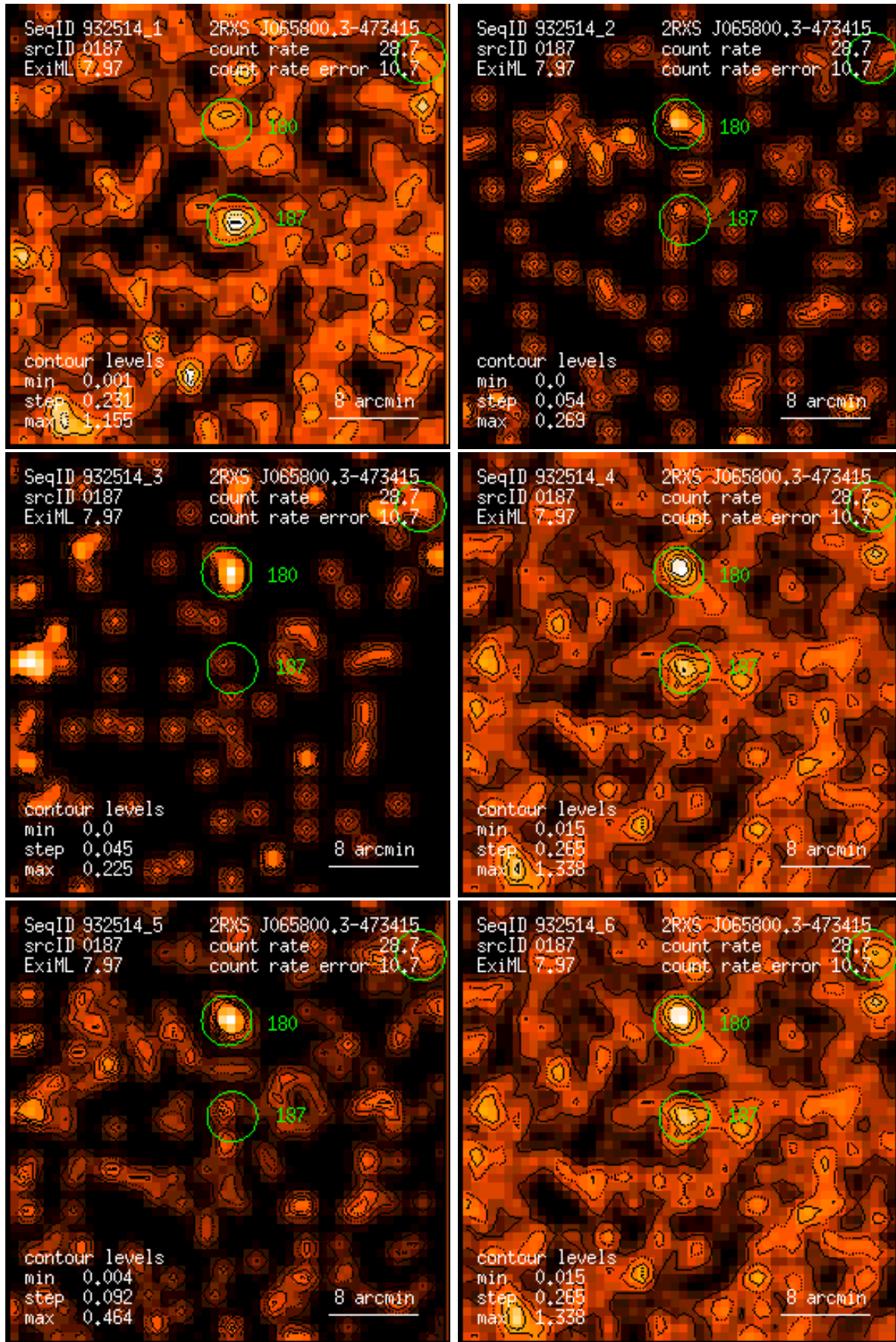
Figure 187: RASS 932514: detection 0187: band rate images, Gaussian filter: (1) PSPC channels 11 – 41, (2) 52 – 90, (3) 91 – 201, (4) 11 – 235, (5) 52 – 201, (6) 11 – 201. Broad band rates in counts/ks. Band rate contour levels in counts/ks/arcmin 2 .
