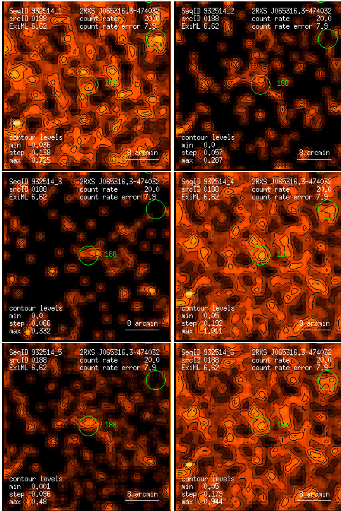
Figure 188: RASS 932514: detection 0188: band rate images, Gaussian filter: (1) PSPC channels 11 – 41, (2) 52 – 90, (3) 91 – 201, (4) 11 – 235, (5) 52 – 201, (6) 11 – 201. Broad band rates in counts/ks. Band rate contour levels in counts/ks/arcmin 2 .
