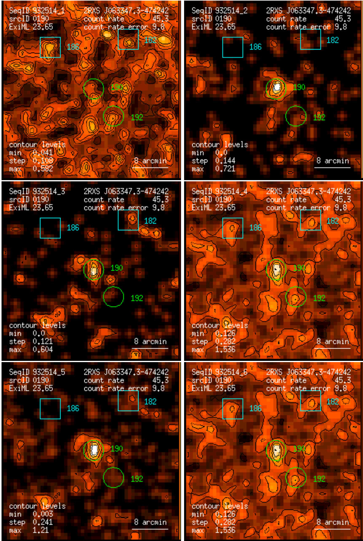
Figure 190: RASS 932514: detection 0190: band rate images, Gaussian filter: (1) PSPC channels 11 – 41, (2) 52 – 90, (3) 91 – 201, (4) 11 – 235, (5) 52 – 201, (6) 11 – 201. Broad band rates in counts/ks. Band rate contour levels in counts/ks/arcmin 2 .
