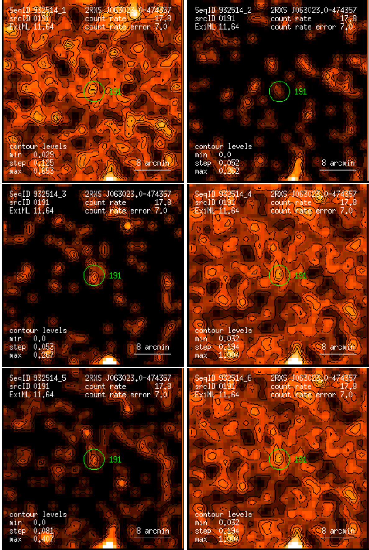
Figure 191: RASS 932514: detection 0191: band rate images, Gaussian filter: (1) PSPC channels 11 – 41, (2) 52 – 90, (3) 91 – 201, (4) 11 – 235, (5) 52 – 201, (6) 11 – 201. Broad band rates in counts/ks. Band rate contour levels in counts/ks/arcmin 2 .
