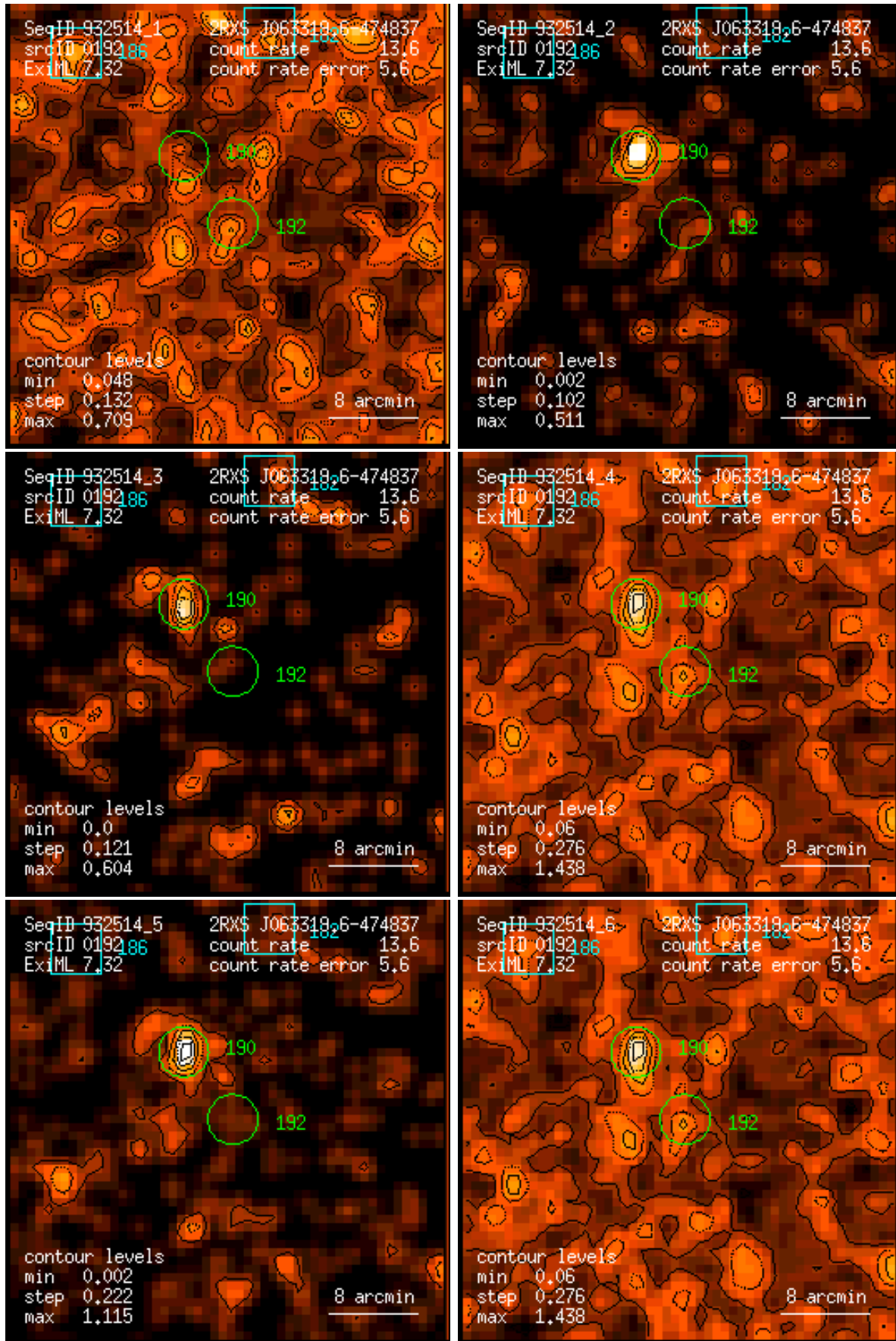
Figure 192: RASS 932514: detection 0192: band rate images, Gaussian filter: (1) PSPC channels 11 – 41, (2) 52 – 90, (3) 91 – 201, (4) 11 – 235, (5) 52 – 201, (6) 11 – 201. Broad band rates in counts/ks. Band rate contour levels in counts/ks/arcmin 2 .
