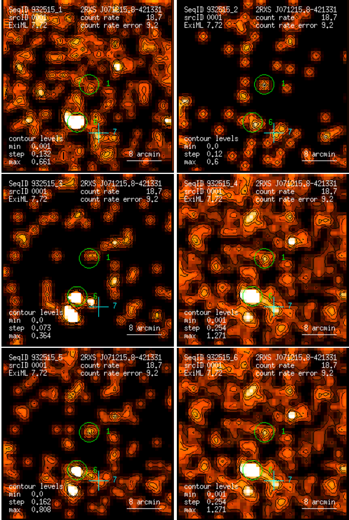
Figure 1: RASS 932515: detection 0001: band rate images, Gaussian filter: (1) PSPC channels 11 – 41, (2) 52 – 90, (3) 91 – 201, (4) 11 – 235, (5) 52 – 201, (6) 11 – 201. Broad band rates in counts/ks. Band rate contour levels in counts/ks/arcmin 2 .
