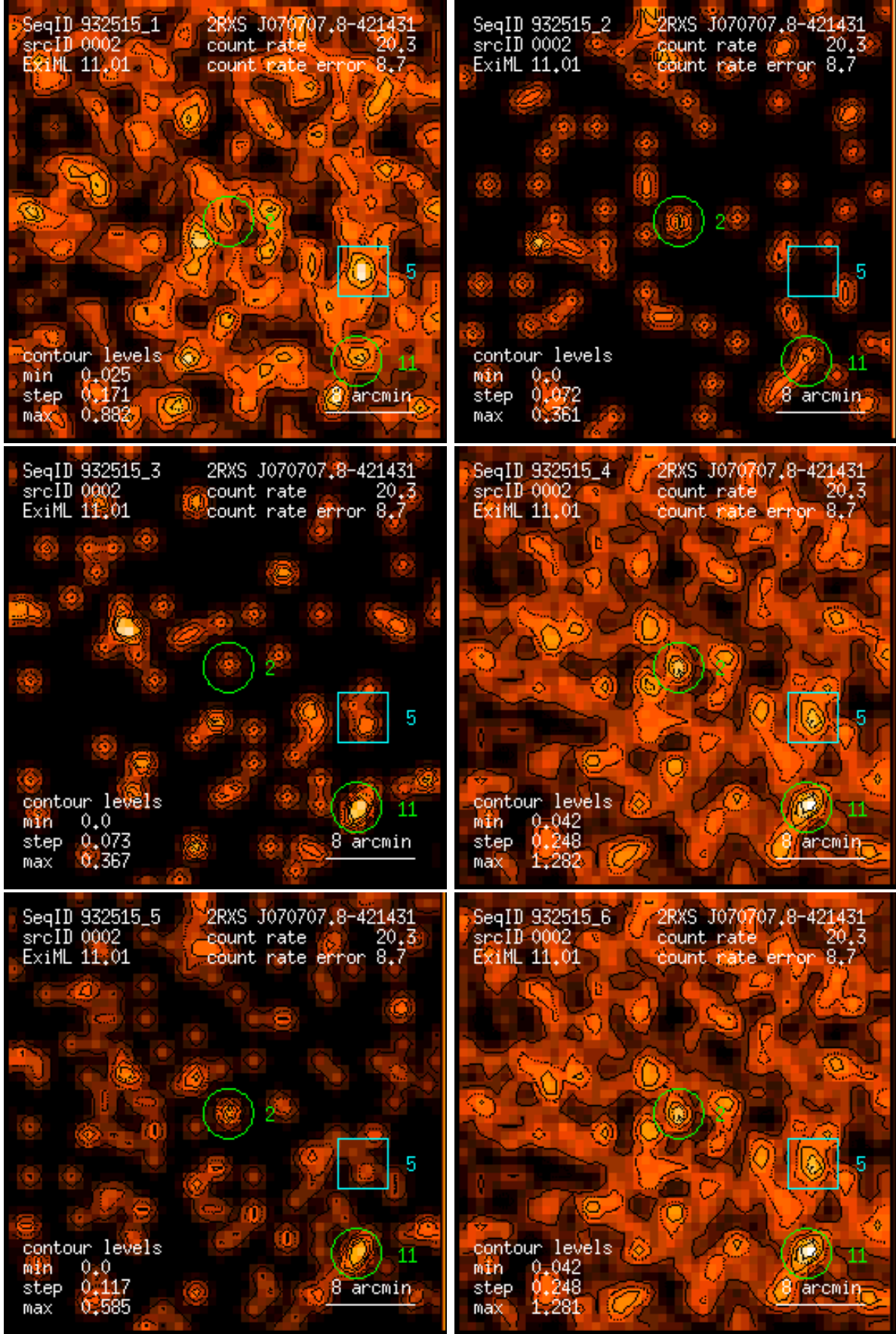
Figure 2: RASS 932515: detection 0002: band rate images, Gaussian filter: (1) PSPC channels 11 – 41, (2) 52 – 90, (3) 91 – 201, (4) 11 – 235, (5) 52 – 201, (6) 11 – 201. Broad band rates in counts/ks. Band rate contour levels in counts/ks/arcmin 2 .
