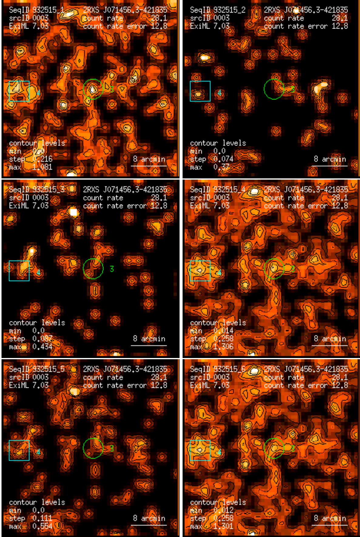
Figure 3: RASS 932515: detection 0003: band rate images, Gaussian filter: (1) PSPC channels 11 – 41, (2) 52 – 90, (3) 91 – 201, (4) 11 – 235, (5) 52 – 201, (6) 11 – 201. Broad band rates in counts/ks. Band rate contour levels in counts/ks/arcmin 2 .
