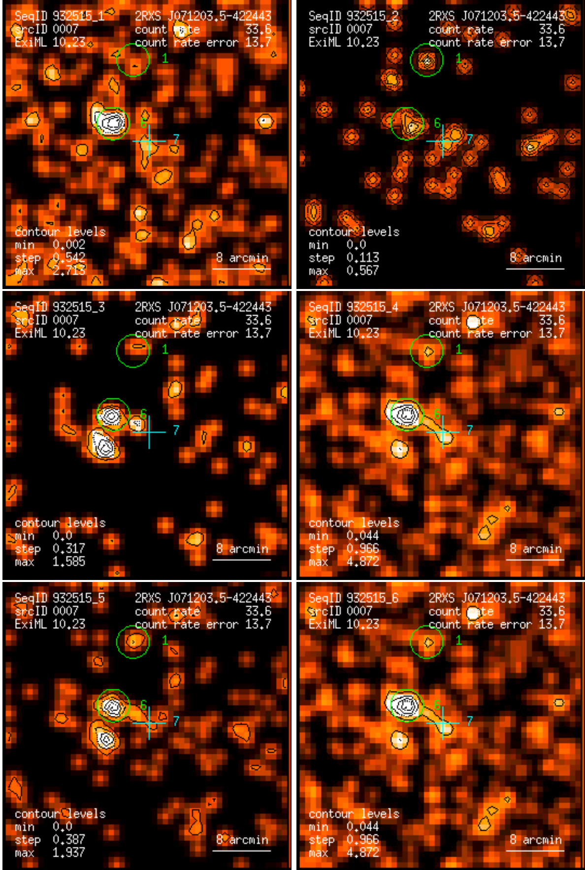
Figure 7: RASS 932515: detection 0007: band rate images, Gaussian filter: (1) PSPC channels 11 – 41, (2) 52 – 90, (3) 91 – 201, (4) 11 – 235, (5) 52 – 201, (6) 11 – 201. Broad band rates in counts/ks. Band rate contour levels in counts/ks/arcmin 2 .
