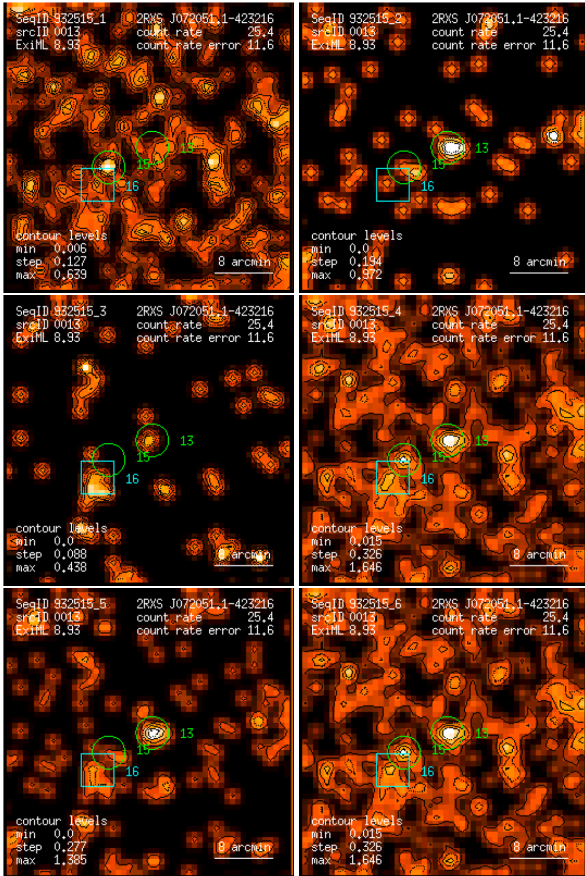
Figure 13: RASS 932515: detection 0013: band rate images, Gaussian filter: (1) PSPC channels 11 – 41, (2) 52 – 90, (3) 91 – 201, (4) 11 – 235, (5) 52 – 201, (6) 11 – 201. Broad band rates in counts/ks. Band rate contour levels in counts/ks/arcmin 2 .
