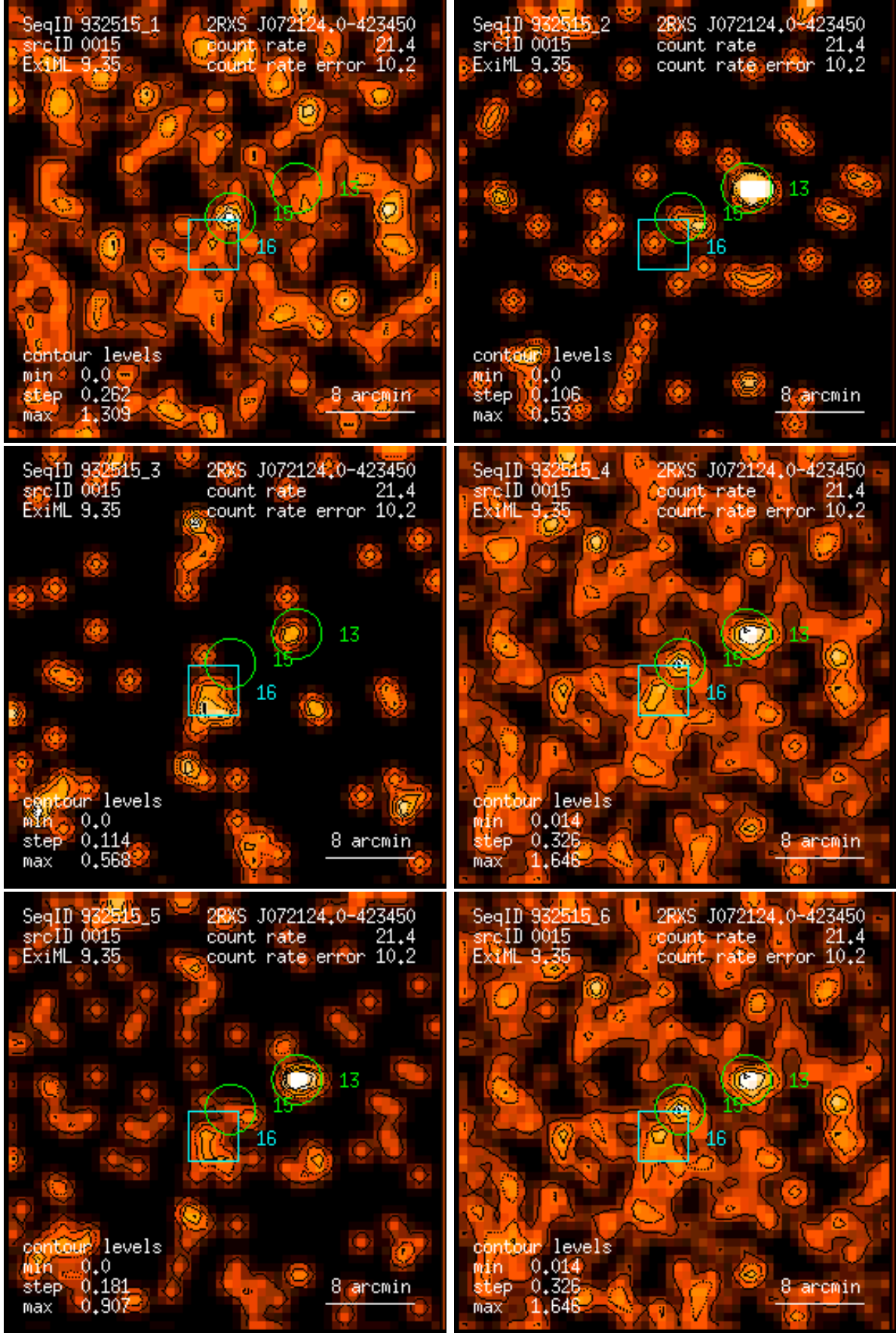
Figure 15: RASS 932515: detection 0015: band rate images, Gaussian filter: (1) PSPC channels 11 – 41, (2) 52 – 90, (3) 91 – 201, (4) 11 – 235, (5) 52 – 201, (6) 11 – 201. Broad band rates in counts/ks. Band rate contour levels in counts/ks/arcmin 2 .
