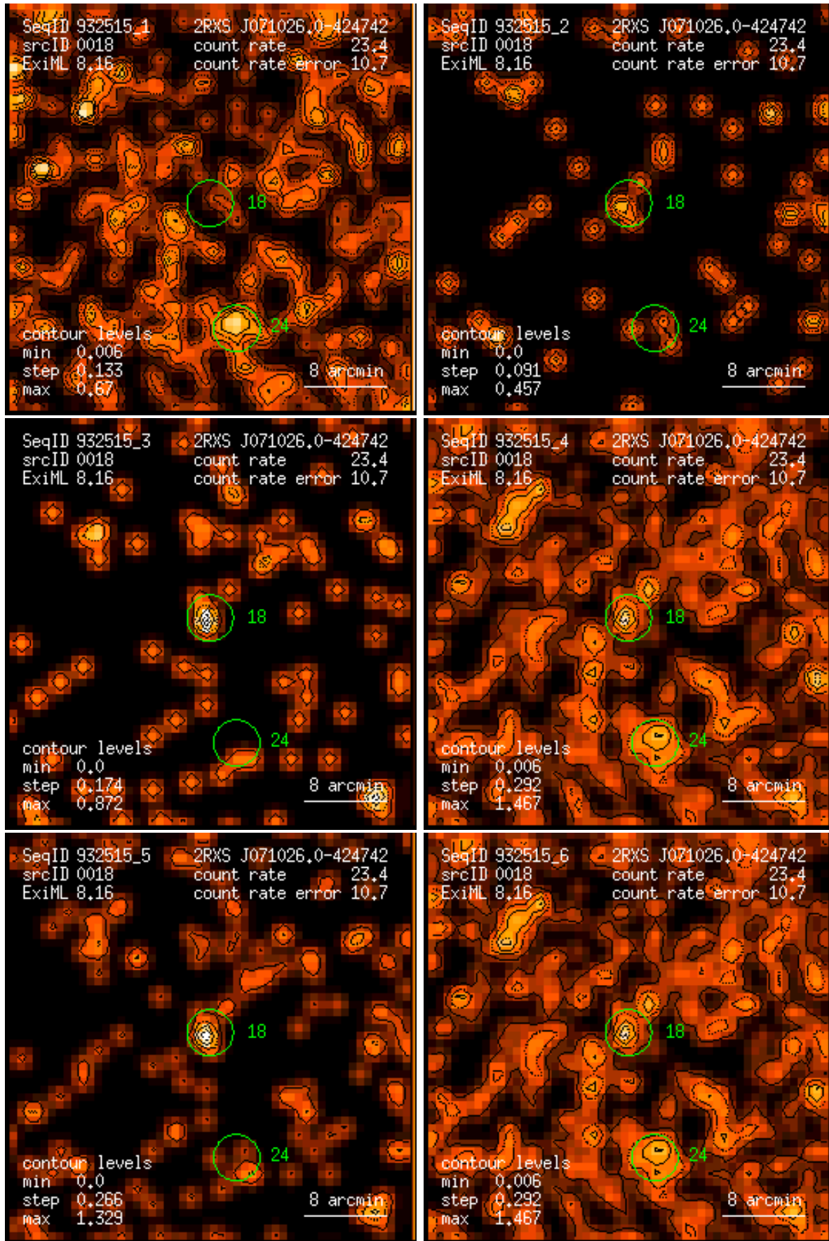
Figure 18: RASS 932515: detection 0018: band rate images, Gaussian filter: (1) PSPC channels 11 – 41, (2) 52 – 90, (3) 91 – 201, (4) 11 – 235, (5) 52 – 201, (6) 11 – 201. Broad band rates in counts/ks. Band rate contour levels in counts/ks/arcmin 2 .
