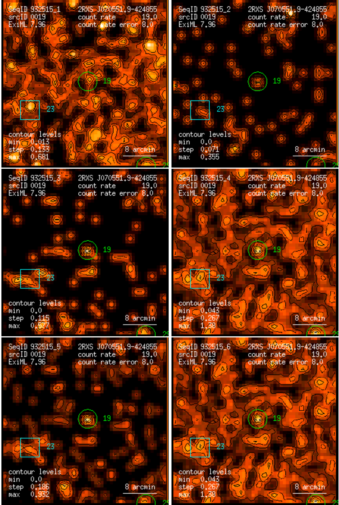
Figure 19: RASS 932515: detection 0019: band rate images, Gaussian filter: (1) PSPC channels 11 – 41, (2) 52 – 90, (3) 91 – 201, (4) 11 – 235, (5) 52 – 201, (6) 11 – 201. Broad band rates in counts/ks. Band rate contour levels in counts/ks/arcmin 2 .
