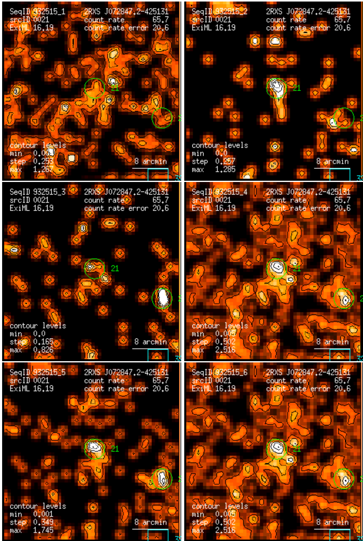
Figure 21: RASS 932515: detection 0021: band rate images, Gaussian filter: (1) PSPC channels 11 – 41, (2) 52 – 90, (3) 91 – 201, (4) 11 – 235, (5) 52 – 201, (6) 11 – 201. Broad band rates in counts/ks. Band rate contour levels in counts/ks/arcmin 2 .
