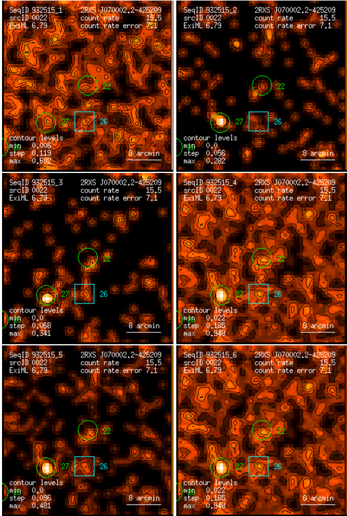
Figure 22: RASS 932515: detection 0022: band rate images, Gaussian filter: (1) PSPC channels 11 – 41, (2) 52 – 90, (3) 91 – 201, (4) 11 – 235, (5) 52 – 201, (6) 11 – 201. Broad band rates in counts/ks. Band rate contour levels in counts/ks/arcmin 2 .
