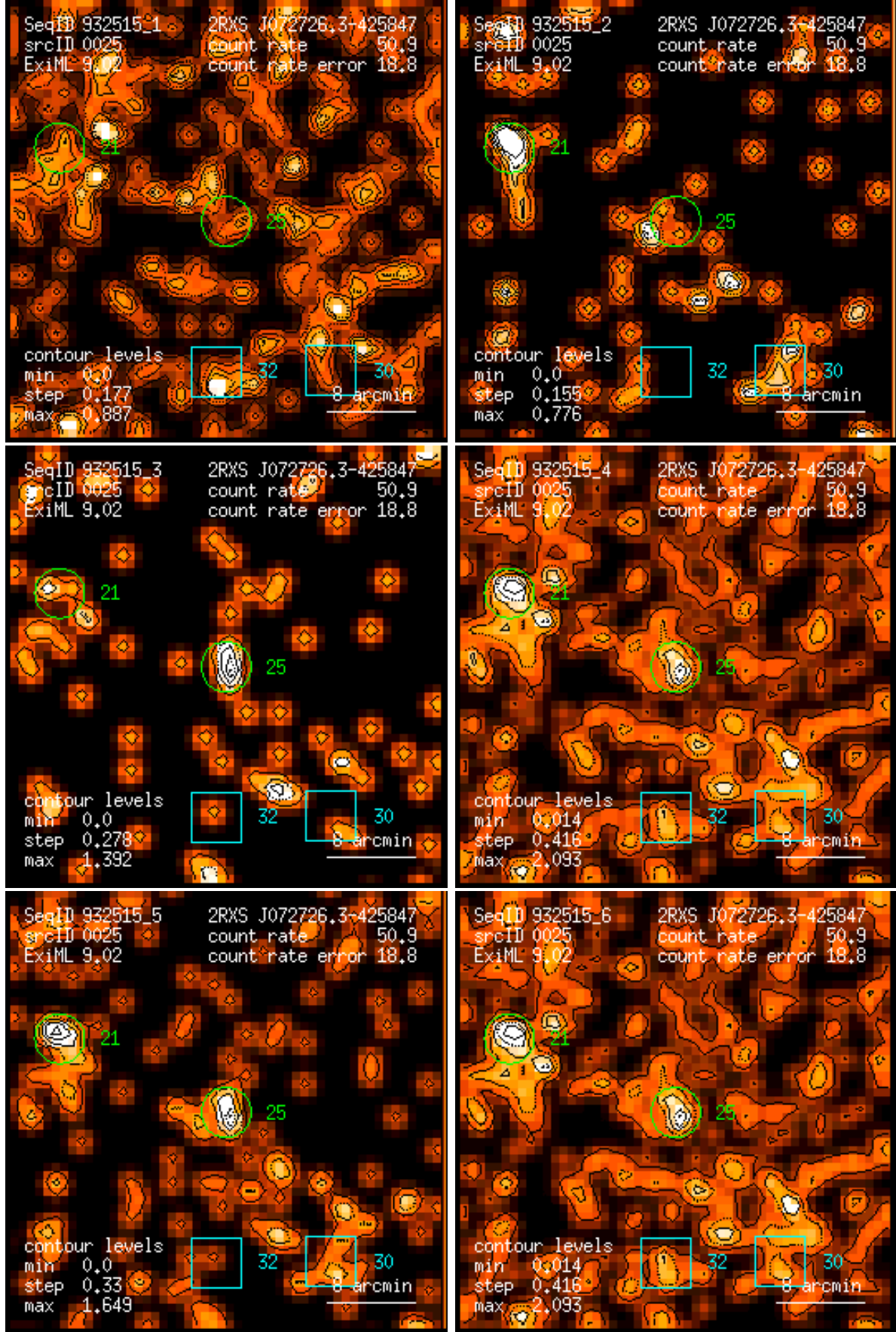
Figure 25: RASS 932515: detection 0025: band rate images, Gaussian filter: (1) PSPC channels 11 – 41, (2) 52 – 90, (3) 91 – 201, (4) 11 – 235, (5) 52 – 201, (6) 11 – 201. Broad band rates in counts/ks. Band rate contour levels in counts/ks/arcmin 2 .
