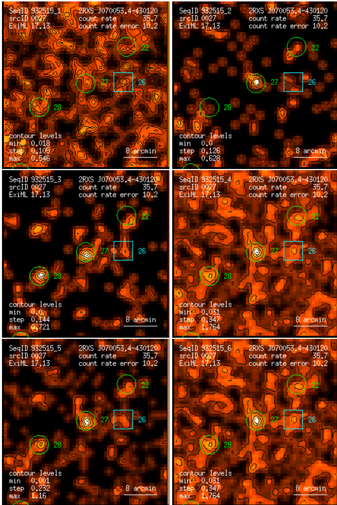
Figure 27: RASS 932515: detection 0027: band rate images, Gaussian filter: (1) PSPC channels 11 – 41, (2) 52 – 90, (3) 91 – 201, (4) 11 – 235, (5) 52 – 201, (6) 11 – 201. Broad band rates in counts/ks. Band rate contour levels in counts/ks/arcmin 2 .
