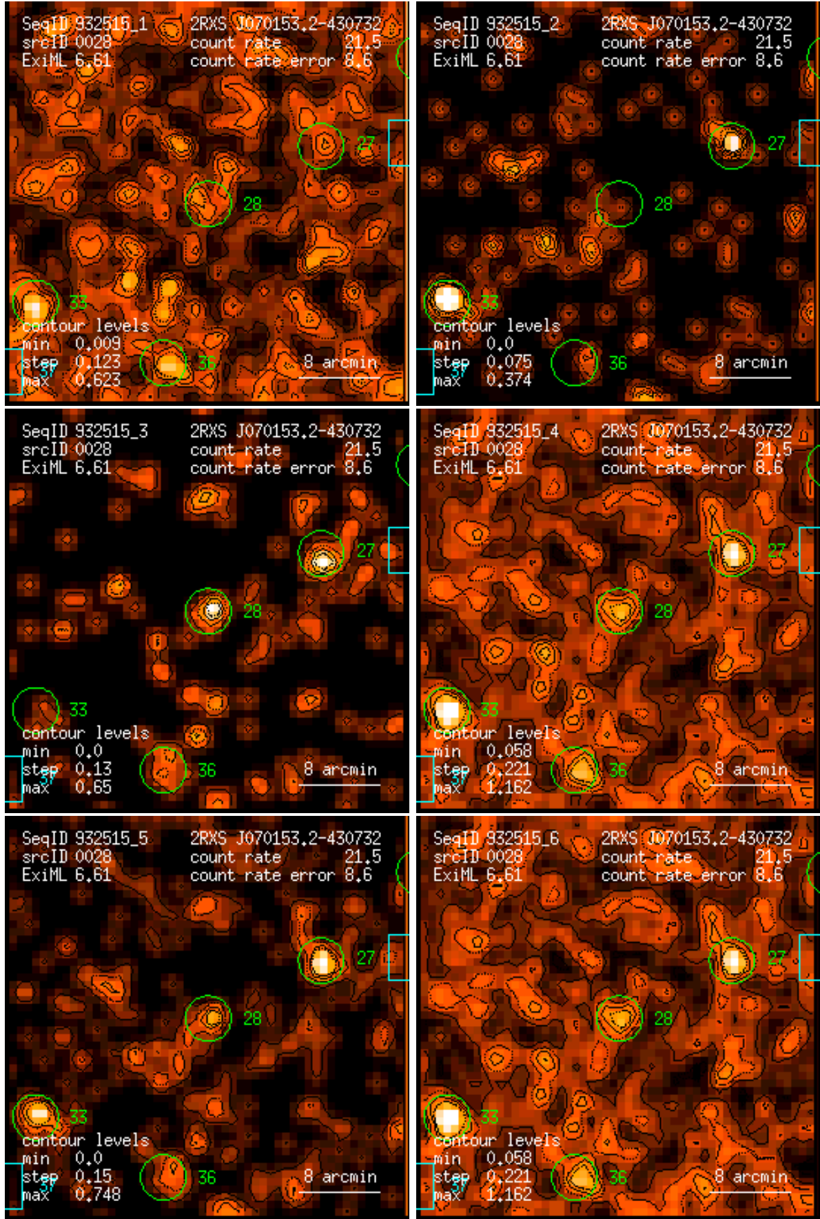
Figure 28: RASS 932515: detection 0028: band rate images, Gaussian filter: (1) PSPC channels 11 – 41, (2) 52 – 90, (3) 91 – 201, (4) 11 – 235, (5) 52 – 201, (6) 11 – 201. Broad band rates in counts/ks. Band rate contour levels in counts/ks/arcmin 2 .
