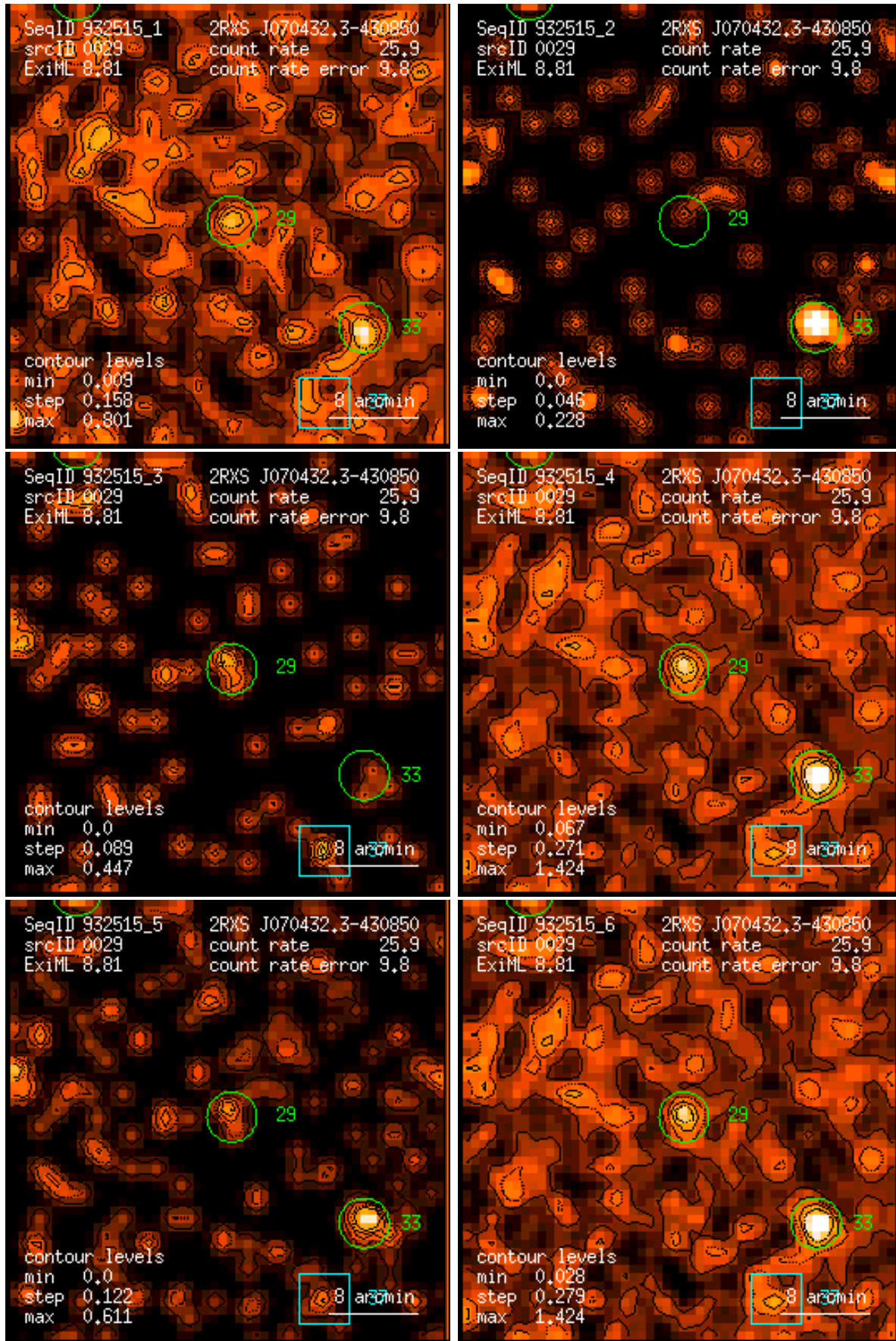
Figure 29: RASS 932515: detection 0029: band rate images, Gaussian filter: (1) PSPC channels 11 – 41, (2) 52 – 90, (3) 91 – 201, (4) 11 – 235, (5) 52 – 201, (6) 11 – 201. Broad band rates in counts/ks. Band rate contour levels in counts/ks/arcmin 2 .
