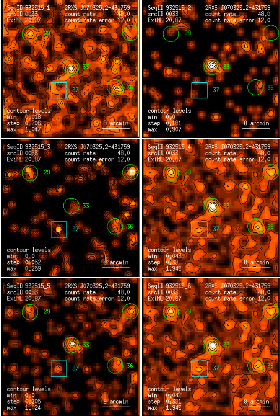
Figure 33: RASS 932515: detection 0033: band rate images, Gaussian filter: (1) PSPC channels 11 – 41, (2) 52 – 90, (3) 91 – 201, (4) 11 – 235, (5) 52 – 201, (6) 11 – 201. Broad band rates in counts/ks. Band rate contour levels in counts/ks/arcmin 2 .
