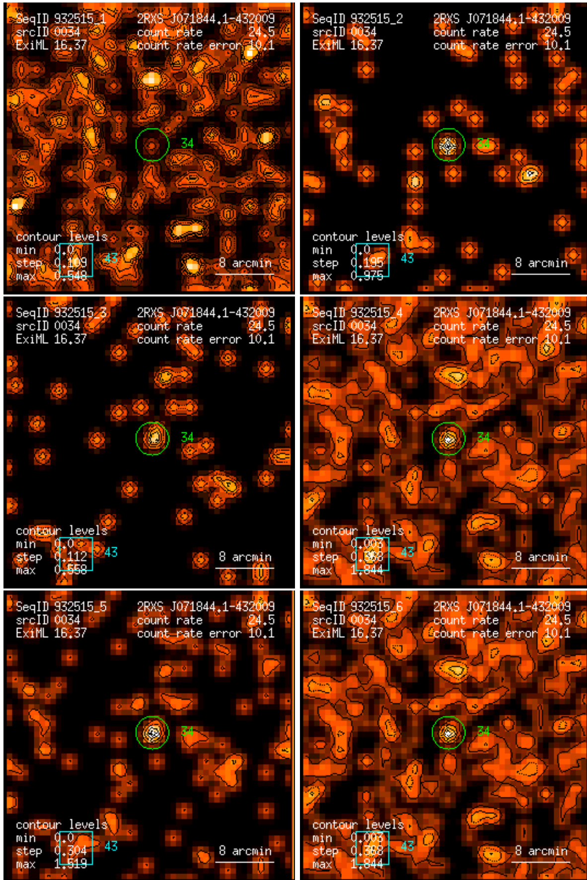
Figure 34: RASS 932515: detection 0034: band rate images, Gaussian filter: (1) PSPC channels 11 – 41, (2) 52 – 90, (3) 91 – 201, (4) 11 – 235, (5) 52 – 201, (6) 11 – 201. Broad band rates in counts/ks. Band rate contour levels in counts/ks/arcmin 2 .
