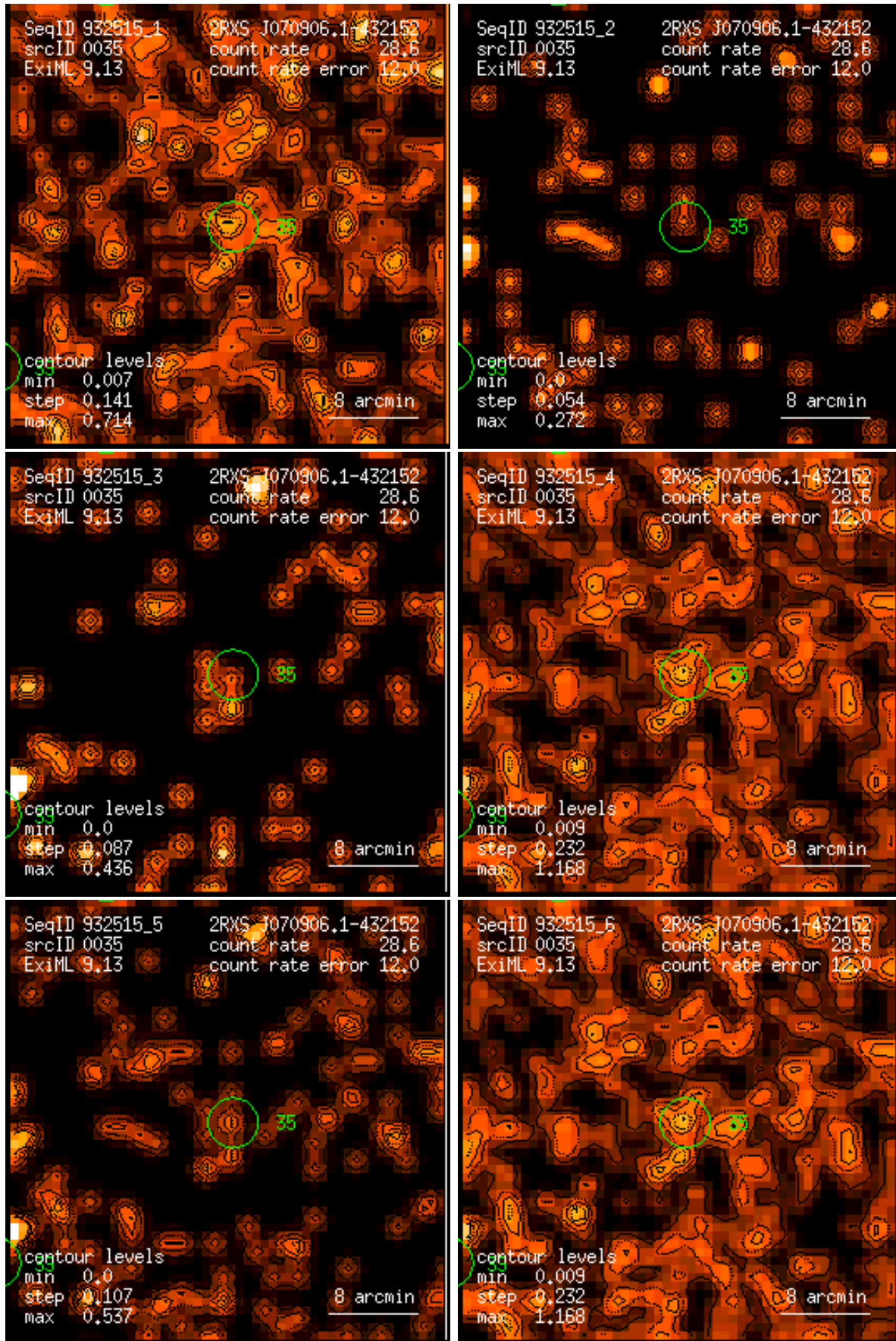
Figure 35: RASS 932515: detection 0035: band rate images, Gaussian filter: (1) PSPC channels 11 – 41, (2) 52 – 90, (3) 91 – 201, (4) 11 – 235, (5) 52 – 201, (6) 11 – 201. Broad band rates in counts/ks. Band rate contour levels in counts/ks/arcmin 2 .
