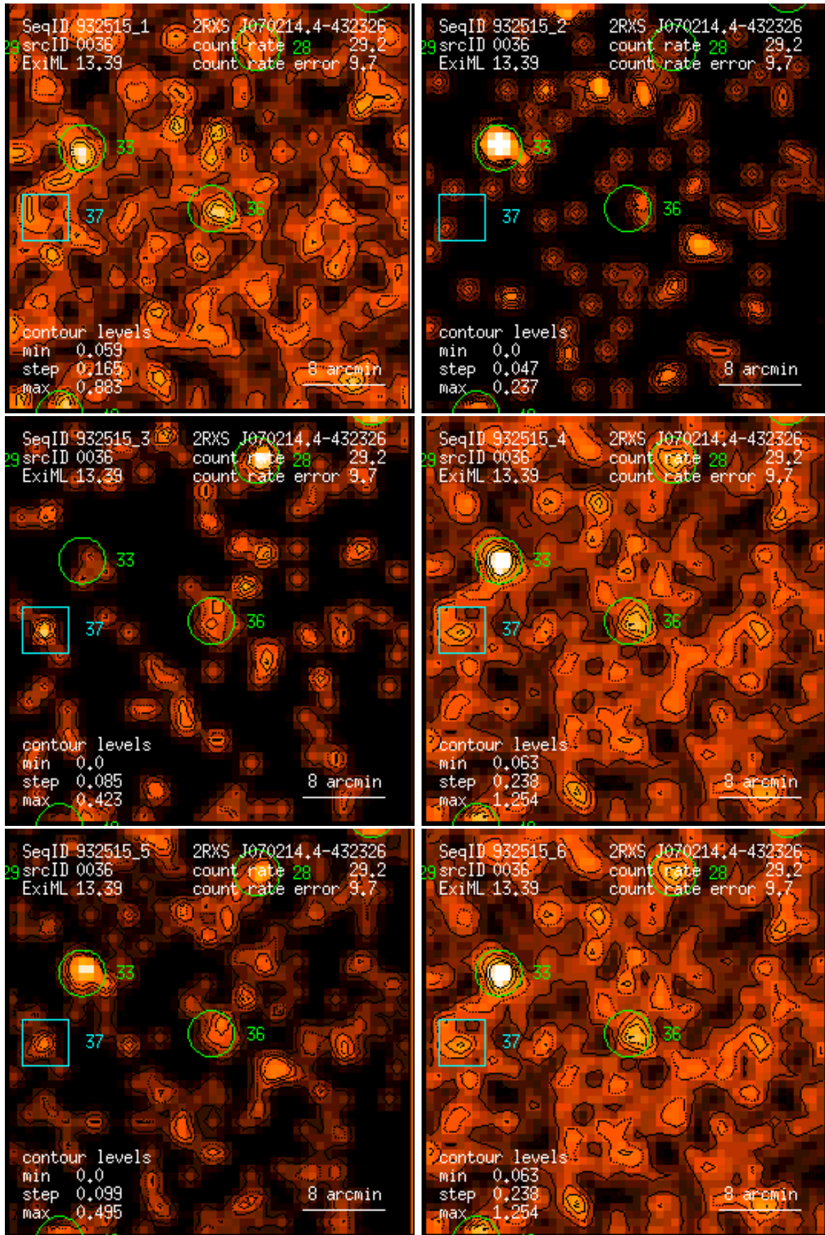
Figure 36: RASS 932515: detection 0036: band rate images, Gaussian filter: (1) PSPC channels 11 – 41, (2) 52 – 90, (3) 91 – 201, (4) 11 – 235, (5) 52 – 201, (6) 11 – 201. Broad band rates in counts/ks. Band rate contour levels in counts/ks/arcmin 2 .
