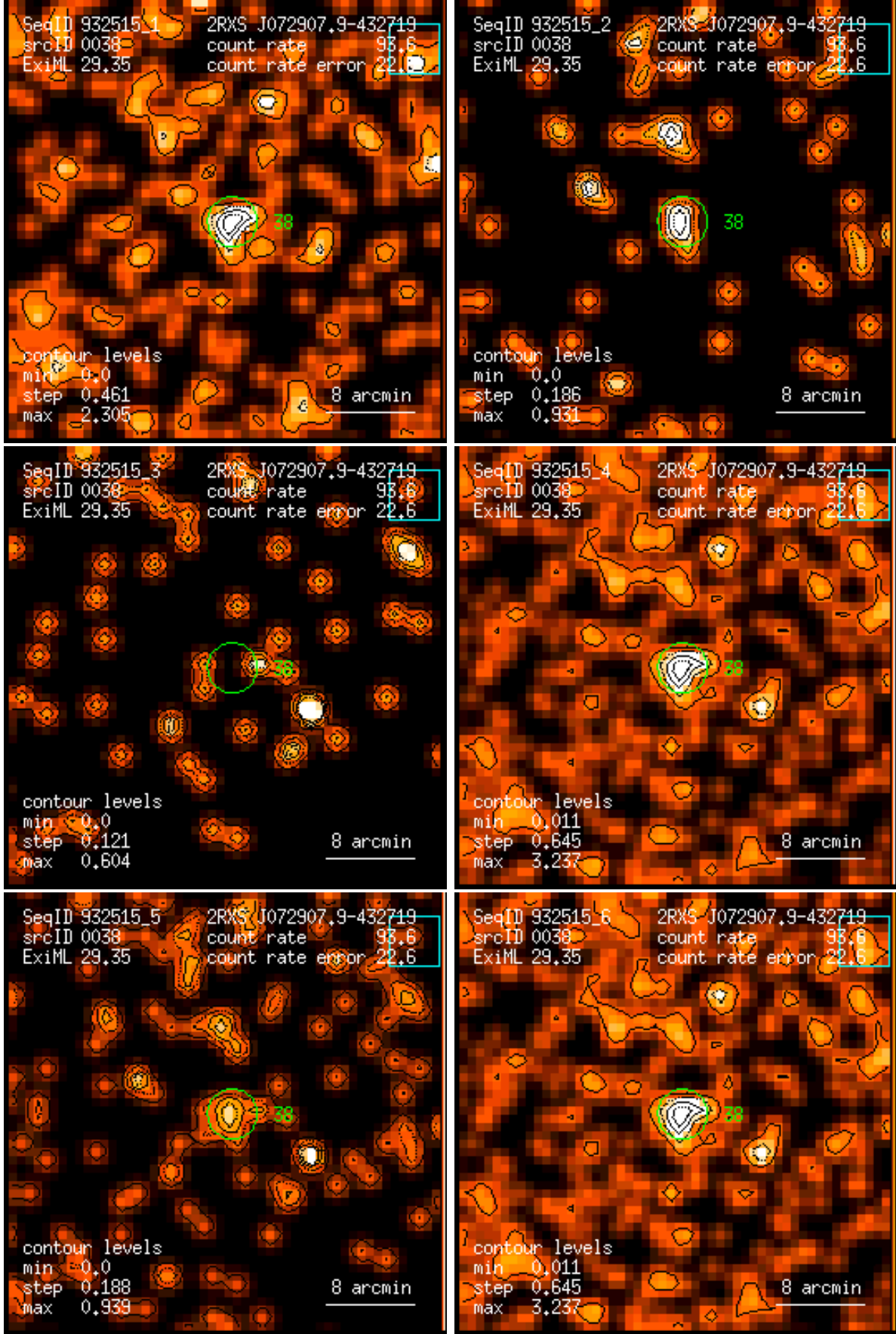
Figure 38: RASS 932515: detection 0038: band rate images, Gaussian filter: (1) PSPC channels 11 – 41, (2) 52 – 90, (3) 91 – 201, (4) 11 – 235, (5) 52 – 201, (6) 11 – 201. Broad band rates in counts/ks. Band rate contour levels in counts/ks/arcmin 2 .
