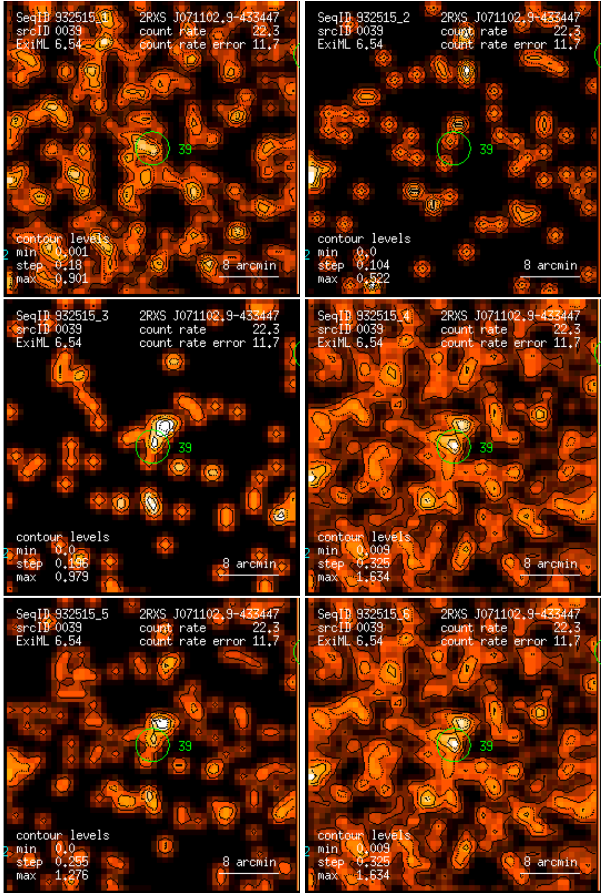
Figure 39: RASS 932515: detection 0039: band rate images, Gaussian filter: (1) PSPC channels 11 – 41, (2) 52 – 90, (3) 91 – 201, (4) 11 – 235, (5) 52 – 201, (6) 11 – 201. Broad band rates in counts/ks. Band rate contour levels in counts/ks/arcmin 2 .
