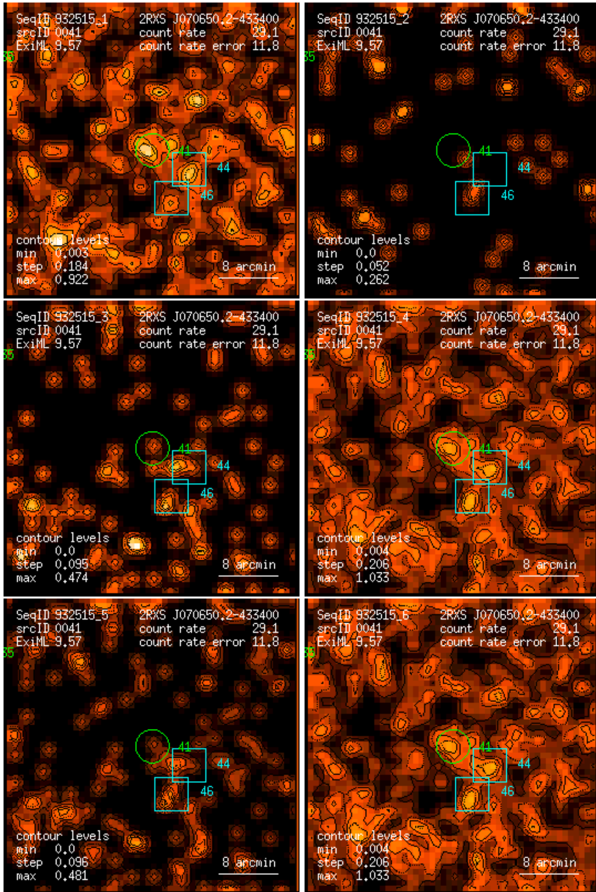
Figure 41: RASS 932515: detection 0041: band rate images, Gaussian filter: (1) PSPC channels 11 – 41, (2) 52 – 90, (3) 91 – 201, (4) 11 – 235, (5) 52 – 201, (6) 11 – 201. Broad band rates in counts/ks. Band rate contour levels in counts/ks/arcmin 2 .
