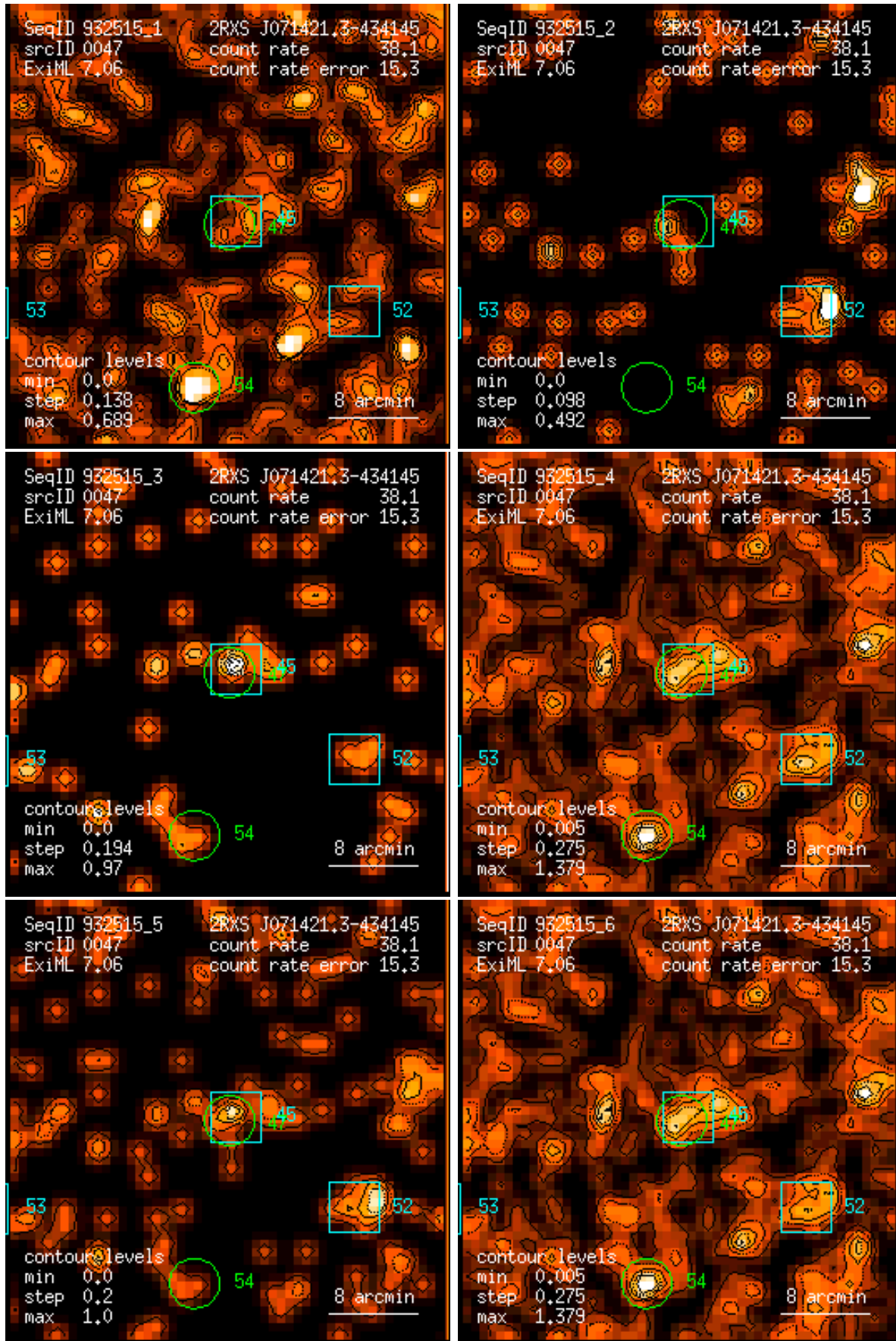
Figure 47: RASS 932515: detection 0047: band rate images, Gaussian filter: (1) PSPC channels 11 – 41, (2) 52 – 90, (3) 91 – 201, (4) 11 – 235, (5) 52 – 201, (6) 11 – 201. Broad band rates in counts/ks. Band rate contour levels in counts/ks/arcmin 2 .
