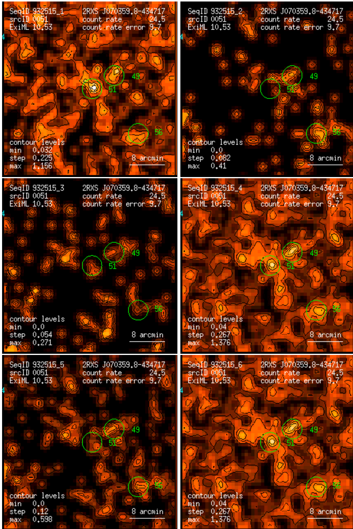
Figure 51: RASS 932515: detection 0051: band rate images, Gaussian filter: (1) PSPC channels 11 – 41, (2) 52 – 90, (3) 91 – 201, (4) 11 – 235, (5) 52 – 201, (6) 11 – 201. Broad band rates in counts/ks. Band rate contour levels in counts/ks/arcmin 2 .
