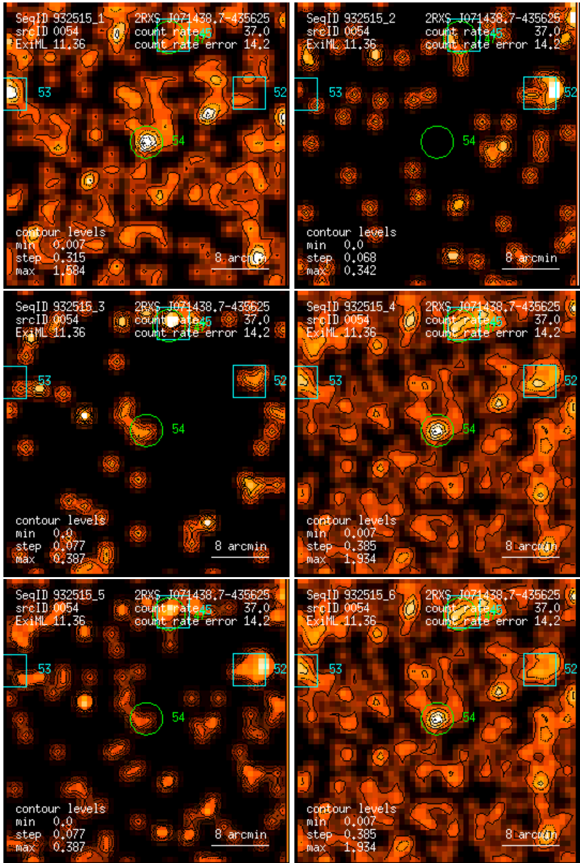
Figure 54: RASS 932515: detection 0054: band rate images, Gaussian filter: (1) PSPC channels 11 – 41, (2) 52 – 90, (3) 91 – 201, (4) 11 – 235, (5) 52 – 201, (6) 11 – 201. Broad band rates in counts/ks. Band rate contour levels in counts/ks/arcmin 2 .
