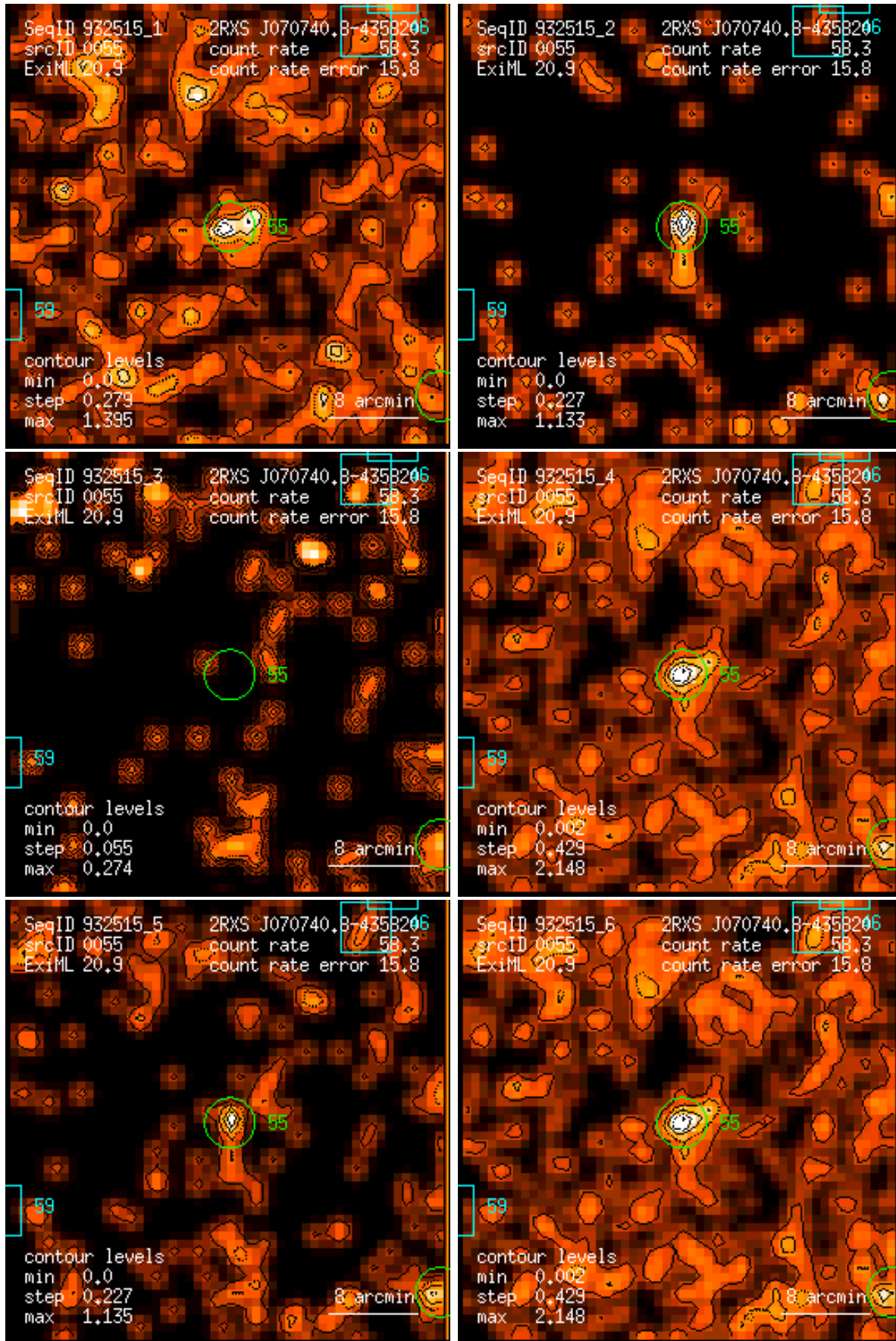
Figure 55: RASS 932515: detection 0055: band rate images, Gaussian filter: (1) PSPC channels 11 – 41, (2) 52 – 90, (3) 91 – 201, (4) 11 – 235, (5) 52 – 201, (6) 11 – 201. Broad band rates in counts/ks. Band rate contour levels in counts/ks/arcmin 2 .
