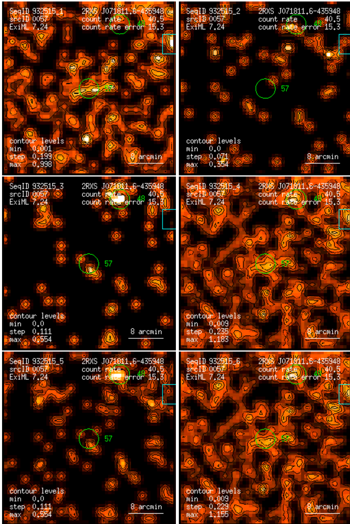
Figure 57: RASS 932515: detection 0057: band rate images, Gaussian filter: (1) PSPC channels 11 – 41, (2) 52 – 90, (3) 91 – 201, (4) 11 – 235, (5) 52 – 201, (6) 11 – 201. Broad band rates in counts/ks. Band rate contour levels in counts/ks/arcmin 2 .
