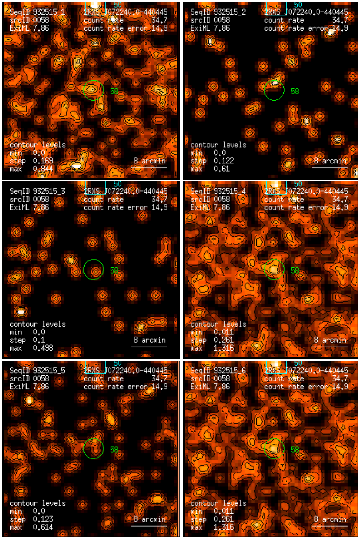
Figure 58: RASS 932515: detection 0058: band rate images, Gaussian filter: (1) PSPC channels 11 – 41, (2) 52 – 90, (3) 91 – 201, (4) 11 – 235, (5) 52 – 201, (6) 11 – 201. Broad band rates in counts/ks. Band rate contour levels in counts/ks/arcmin 2 .
