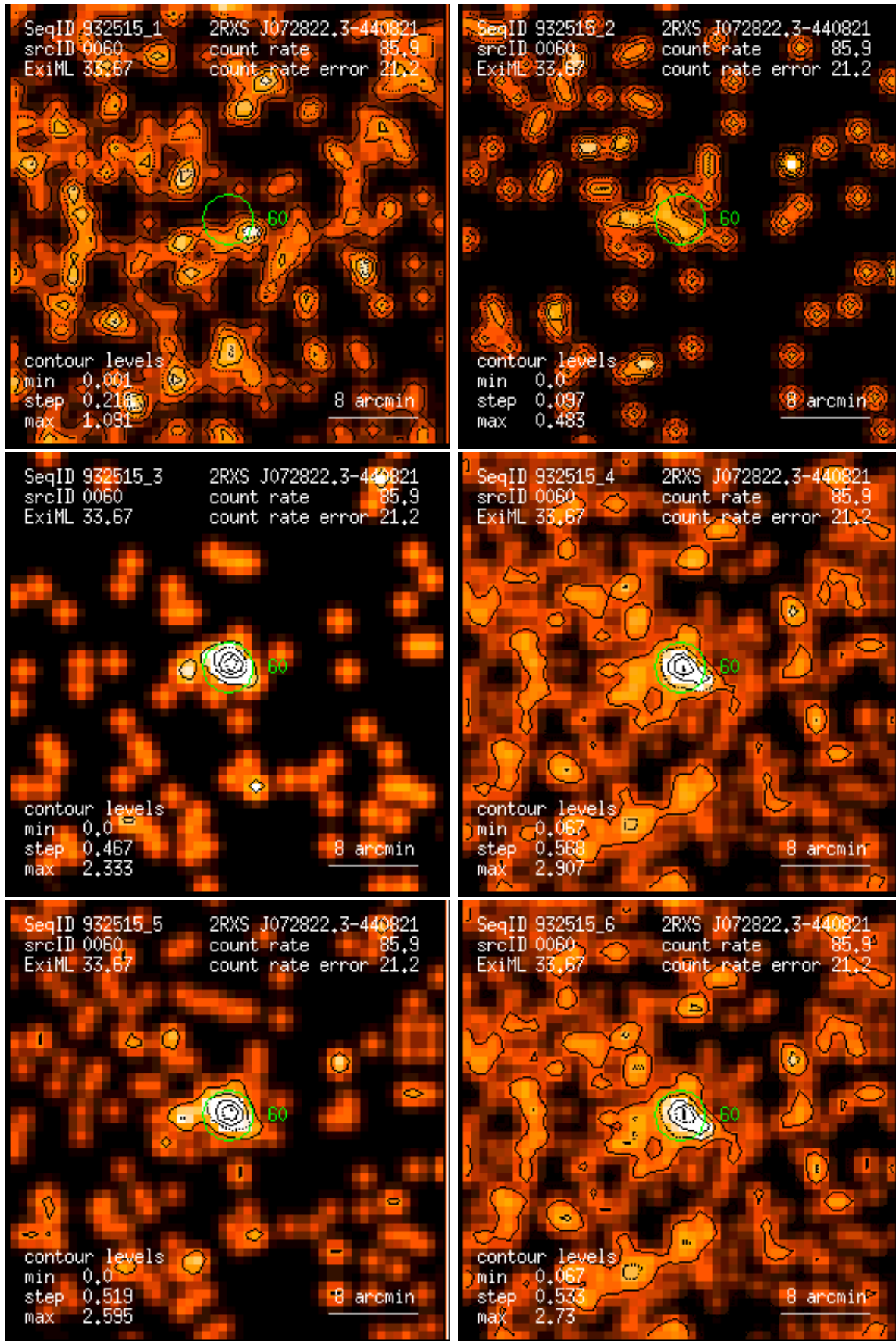
Figure 60: RASS 932515: detection 0060: band rate images, Gaussian filter: (1) PSPC channels 11 – 41, (2) 52 – 90, (3) 91 – 201, (4) 11 – 235, (5) 52 – 201, (6) 11 – 201. Broad band rates in counts/ks. Band rate contour levels in counts/ks/arcmin 2 .
