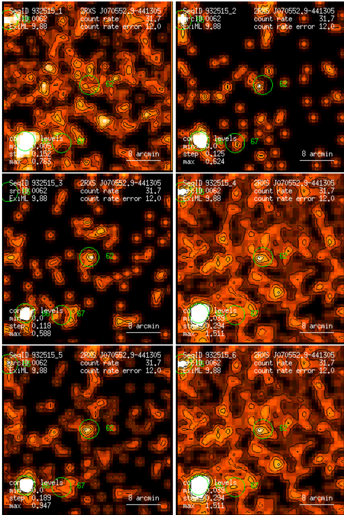
Figure 62: RASS 932515: detection 0062: band rate images, Gaussian filter: (1) PSPC channels 11 – 41, (2) 52 – 90, (3) 91 – 201, (4) 11 – 235, (5) 52 – 201, (6) 11 – 201. Broad band rates in counts/ks. Band rate contour levels in counts/ks/arcmin 2 .
