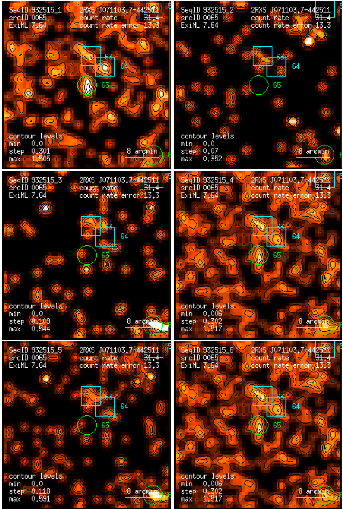
Figure 65: RASS 932515: detection 0065: band rate images, Gaussian filter: (1) PSPC channels 11 – 41, (2) 52 – 90, (3) 91 – 201, (4) 11 – 235, (5) 52 – 201, (6) 11 – 201. Broad band rates in counts/ks. Band rate contour levels in counts/ks/arcmin 2 .
