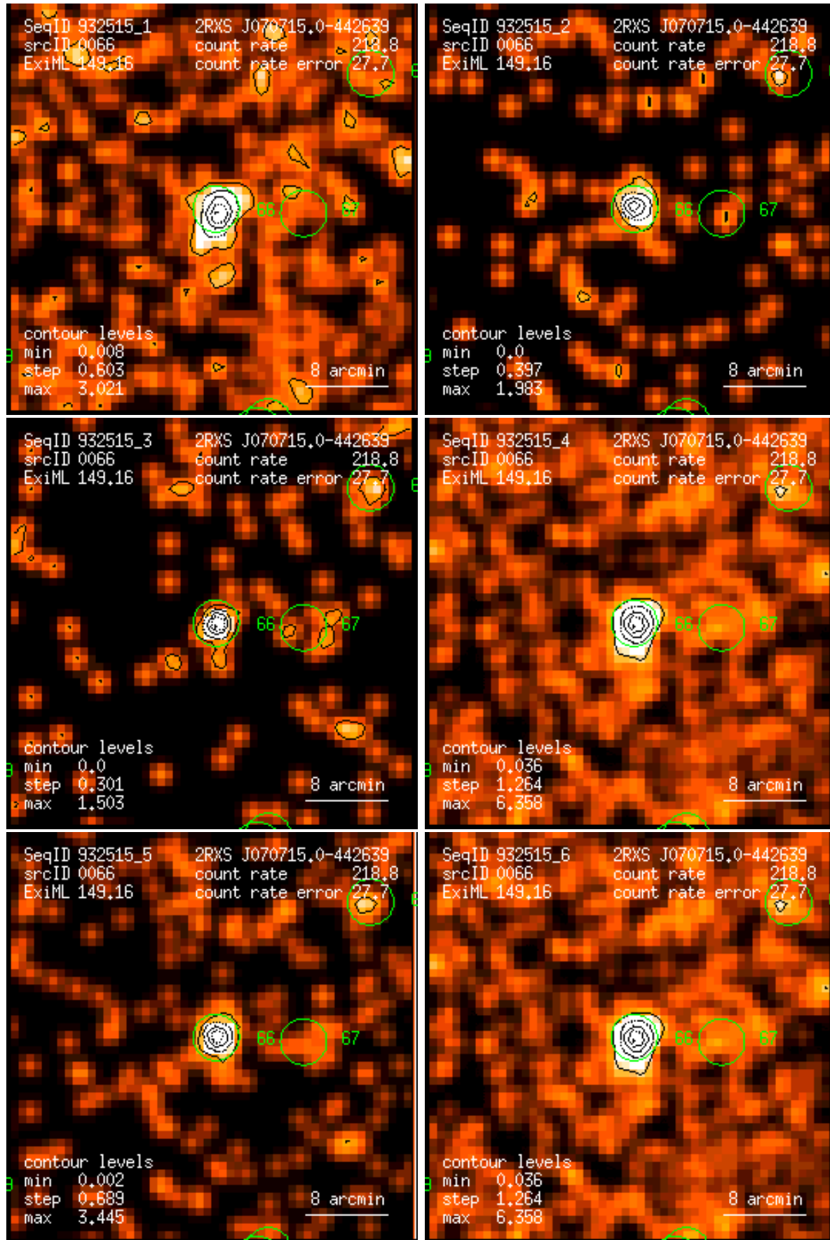
Figure 66: RASS 932515: detection 0066: band rate images, Gaussian filter: (1) PSPC channels 11 – 41, (2) 52 – 90, (3) 91 – 201, (4) 11 – 235, (5) 52 – 201, (6) 11 – 201. Broad band rates in counts/ks. Band rate contour levels in counts/ks/arcmin 2 .
