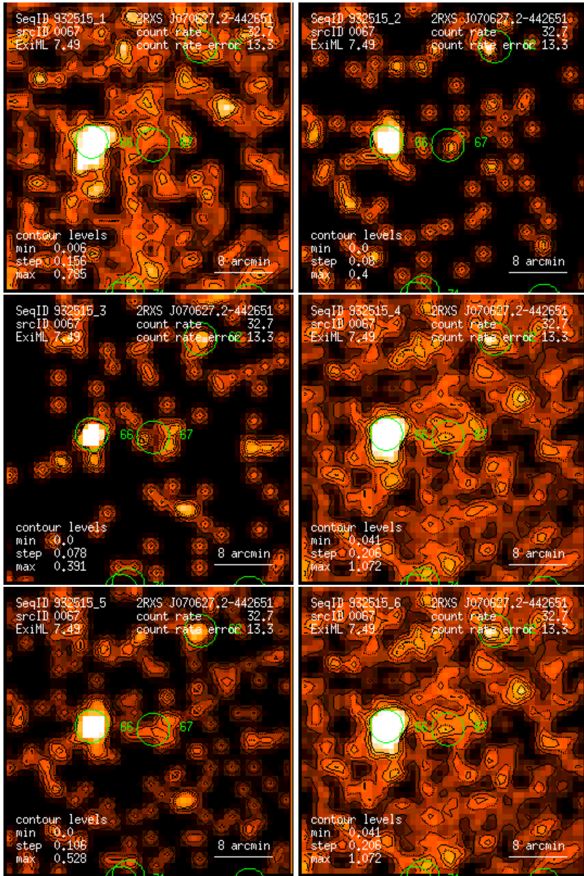
Figure 67: RASS 932515: detection 0067: band rate images, Gaussian filter: (1) PSPC channels 11 – 41, (2) 52 – 90, (3) 91 – 201, (4) 11 – 235, (5) 52 – 201, (6) 11 – 201. Broad band rates in counts/ks. Band rate contour levels in counts/ks/arcmin 2 .
