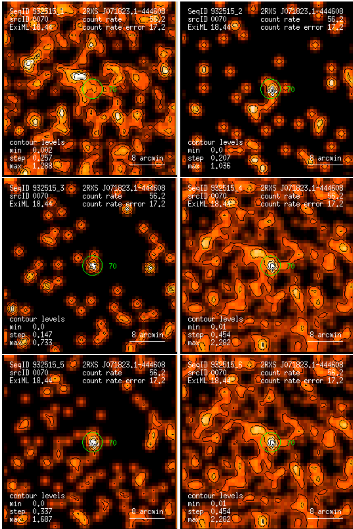
Figure 70: RASS 932515: detection 0070: band rate images, Gaussian filter: (1) PSPC channels 11 – 41, (2) 52 – 90, (3) 91 – 201, (4) 11 – 235, (5) 52 – 201, (6) 11 – 201. Broad band rates in counts/ks. Band rate contour levels in counts/ks/arcmin 2 .
