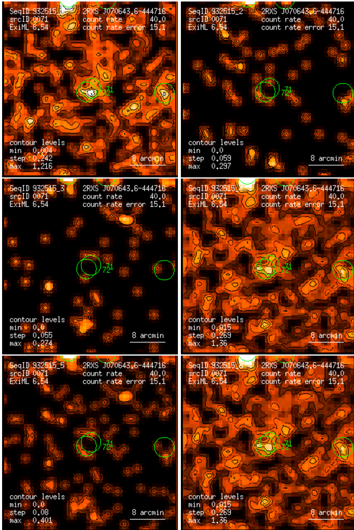
Figure 71: RASS 932515: detection 0071: band rate images, Gaussian filter: (1) PSPC channels 11 – 41, (2) 52 – 90, (3) 91 – 201, (4) 11 – 235, (5) 52 – 201, (6) 11 – 201. Broad band rates in counts/ks. Band rate contour levels in counts/ks/arcmin 2 .
