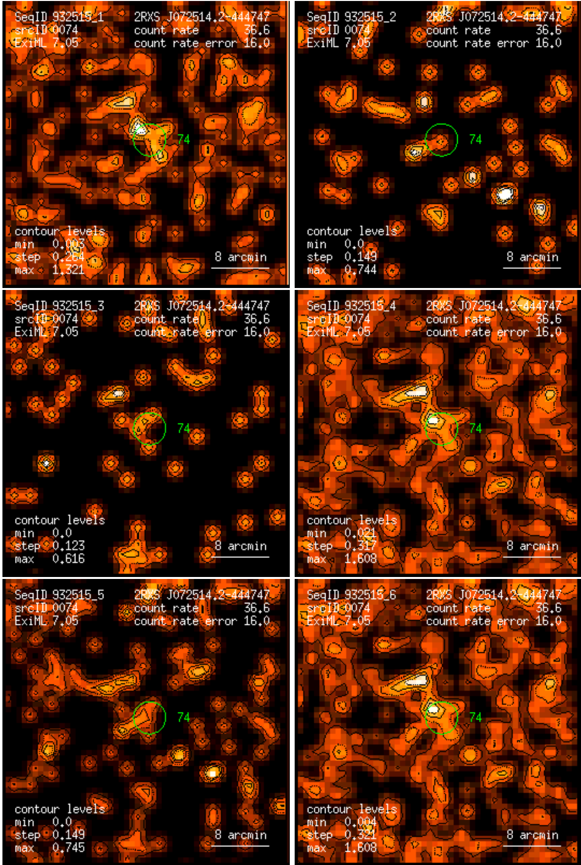
Figure 74: RASS 932515: detection 0074: band rate images, Gaussian filter: (1) PSPC channels 11 – 41, (2) 52 – 90, (3) 91 – 201, (4) 11 – 235, (5) 52 – 201, (6) 11 – 201. Broad band rates in counts/ks. Band rate contour levels in counts/ks/arcmin 2 .
