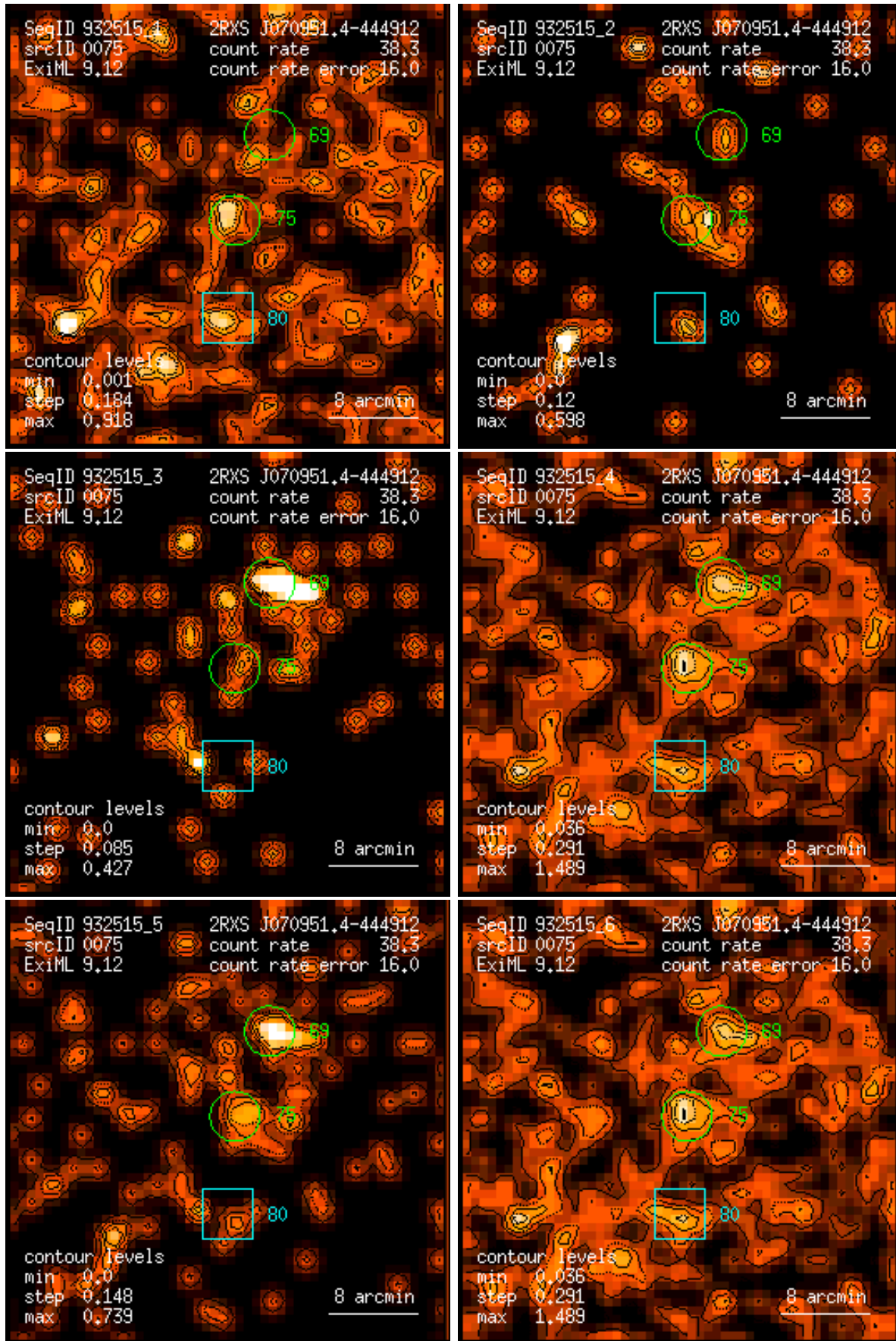
Figure 75: RASS 932515: detection 0075: band rate images, Gaussian filter: (1) PSPC channels 11 – 41, (2) 52 – 90, (3) 91 – 201, (4) 11 – 235, (5) 52 – 201, (6) 11 – 201. Broad band rates in counts/ks. Band rate contour levels in counts/ks/arcmin 2 .
