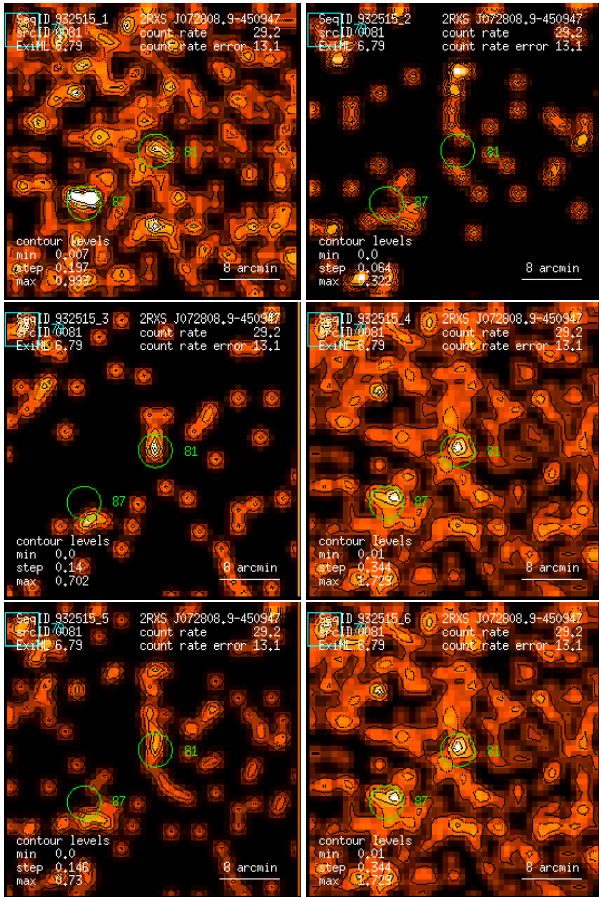
Figure 81: RASS 932515: detection 0081: band rate images, Gaussian filter: (1) PSPC channels 11 – 41, (2) 52 – 90, (3) 91 – 201, (4) 11 – 235, (5) 52 – 201, (6) 11 – 201. Broad band rates in counts/ks. Band rate contour levels in counts/ks/arcmin 2 .
